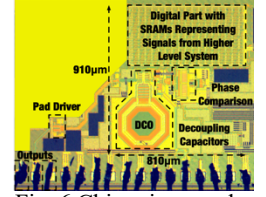
Fig. 6 Chip micrograph.
