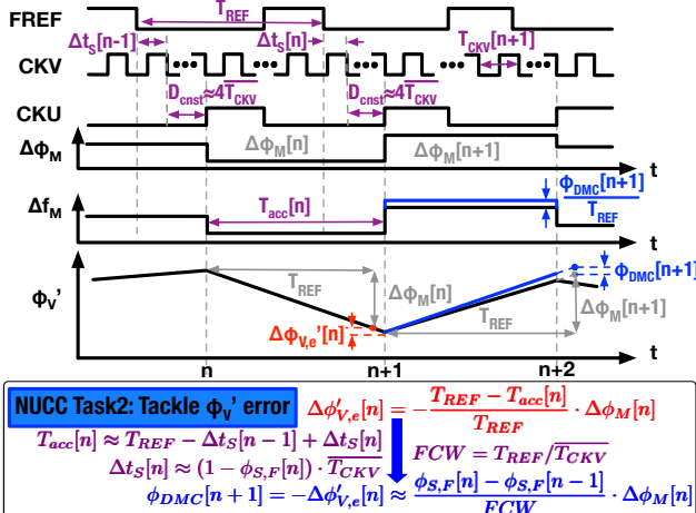
Fig. 2: Conceptual NUCC operation: estimating PM error ( \Delta\phi'_{v,e} ) due to time-variant T_{\text{acc}} and compensating it with \phi_{\text{DMC}} in the next cycle.
