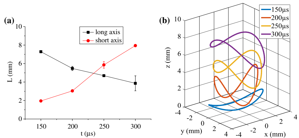
Fig. 10 Front vortex ring characteristics. a Variation of axial length; b shape transformation during propagation
