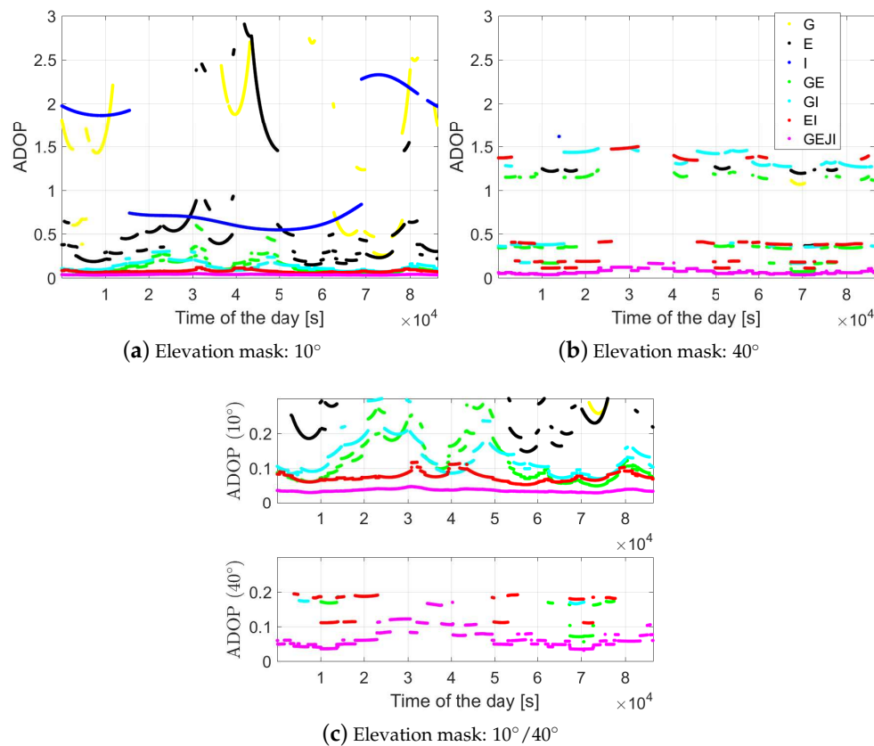
Figure 5. ADOP (Equation (10)) of baseline CUAU-CUCC on DOY 224, 2018 with elevation masks of 10 (a); 40 degrees (b) and the figures zoomed out for small ADOP values (c). The data sampling rate is 1 Hz.
