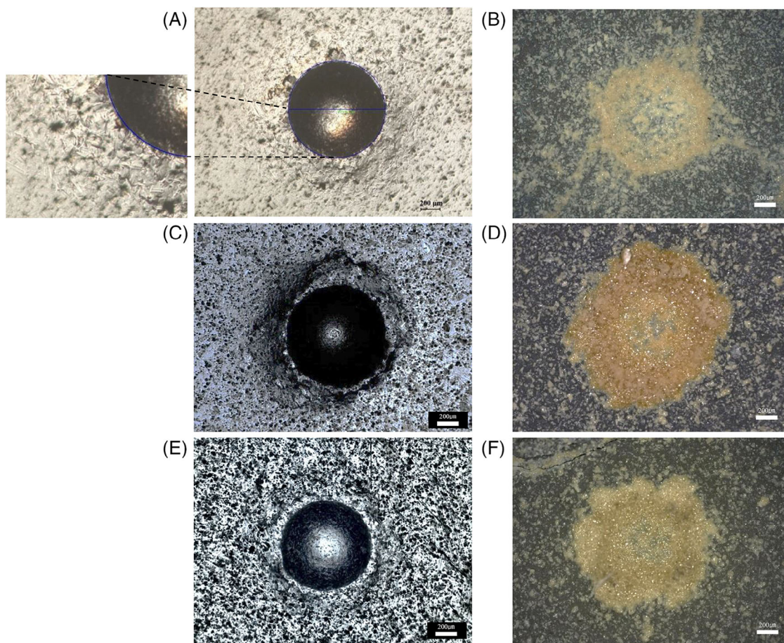
FIGURE 4 Digital micrographs of \text{Ti}_2\text{AlC} crack and damage: (A) Before healing at 1000^\circ\text{C} , (B) after healing at 1000^\circ\text{C} , (C) before healing at 1200^\circ\text{C} , (D) after healing at 1200^\circ\text{C} , (E) before healing at 1400^\circ\text{C} , and (F) after healing at 1400^\circ\text{C} for 2 h in air after indentation test with a load of 3000N using WC spherical indenter in a radius of 1.98 mm.
