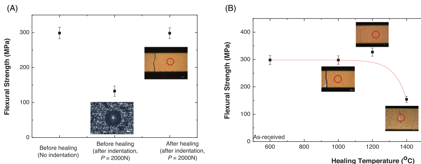
FIGURE 11 (A) Four-point bending test results of the original \text{Ti}_2\text{AlC} bar sample, the sample containing quasi-plastic damage and the sample containing the damage and posthealed. (B) Four-point bending test results before and after healing at each different temperature for 2 h.
