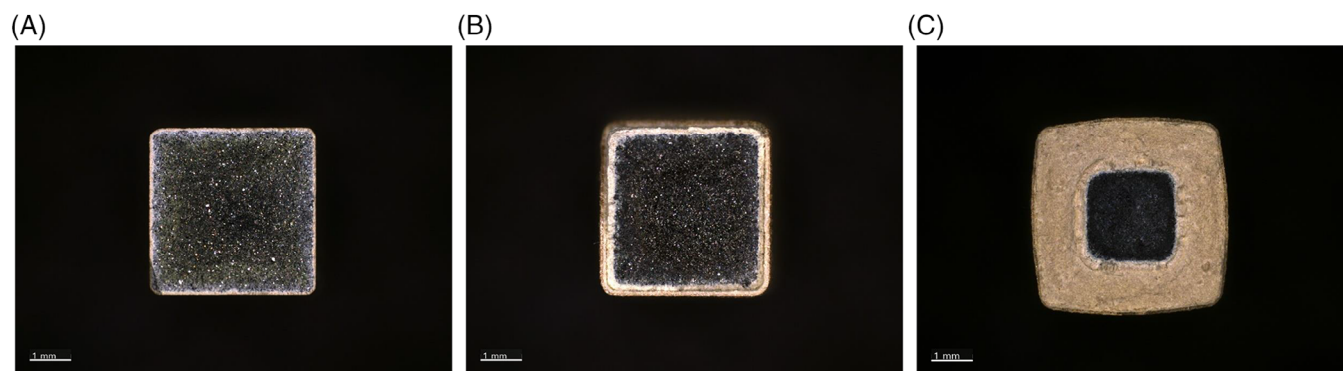
FIGURE 5 Digital micrographs of the fractured surface of \text{Ti}_2\text{AlC} after healing at different temperatures: (A) 1000^\circ\text{C} , (B) 1200^\circ\text{C} , and (C) 1400^\circ\text{C} for 2 h in air.
