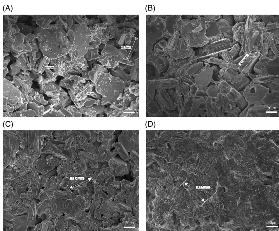
FIGURE 8 SEM micrographs of the fracture surface of \text{Ti}_2\text{AlC} (A) before healing, (B) after healing at 1000^\circ\text{C} , (C) after healing at 1200^\circ\text{C} , and (D) after healing at 1400^\circ\text{C} for 2 h in air.
