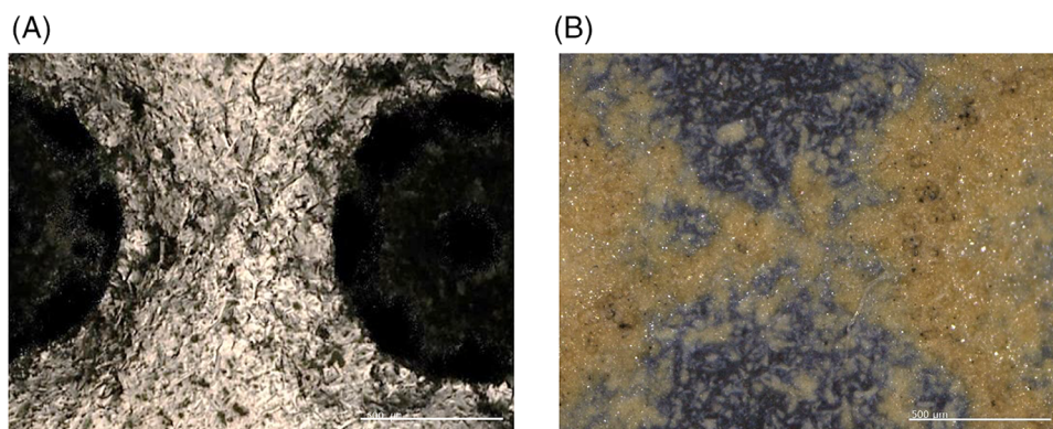
FIGURE 7 Indentation damage and microcracks on \text{Ti}_2\text{AlC} bulk sample using a WC ball with a radius of 1.98 mm and a load of 3000N. (A) The microcracks between two indentation damage sites coalesced and (B) the oxides filled the radial crack and damages due to heat treatment after healing test at 1000^\circ\text{C} for 2 h in the air.
