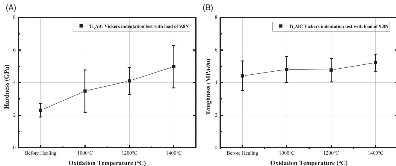
FIGURE 12 (A) Vickers hardness and (B) fracture toughness results with a load of P = 9.8\text{N} on \text{Ti}_2\text{AlC} bulk samples after healing at 1000, 1200, and 1400°C for 2 h in air. The graph also includes the data of \text{Ti}_2\text{AlC} bulk samples before healing.
