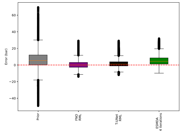
Fig. 21. Box plots comparing monitoring pressure errors between standard RML and Hybrid-RML-Surrogate using FNO and T-UNet surrogates.
