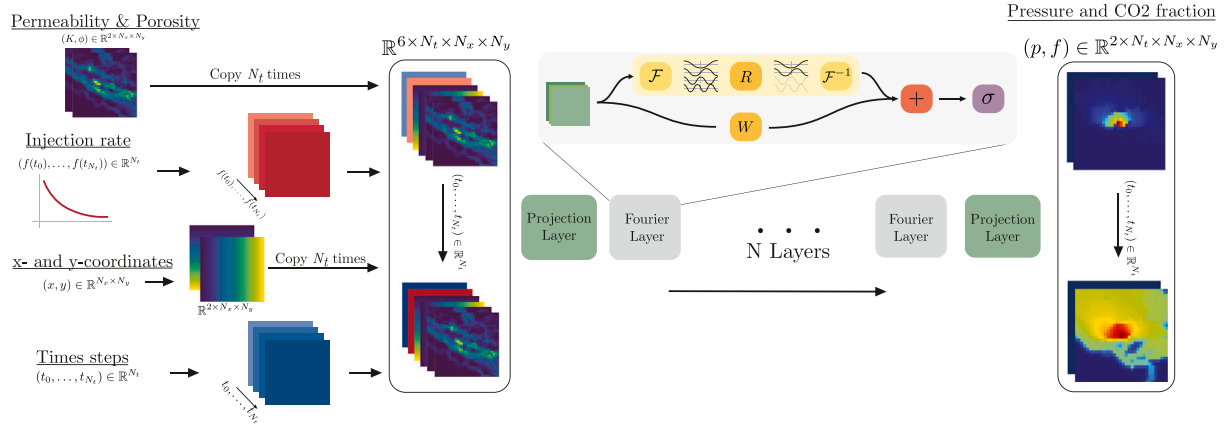
Fig. 5. FNO architecture.
