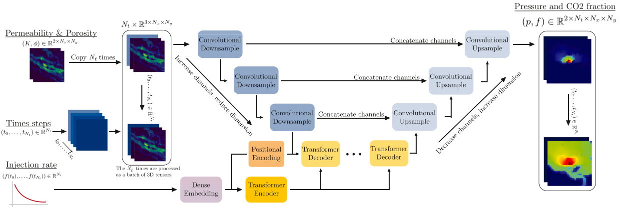
Fig. 4. T-UNet architecture.
