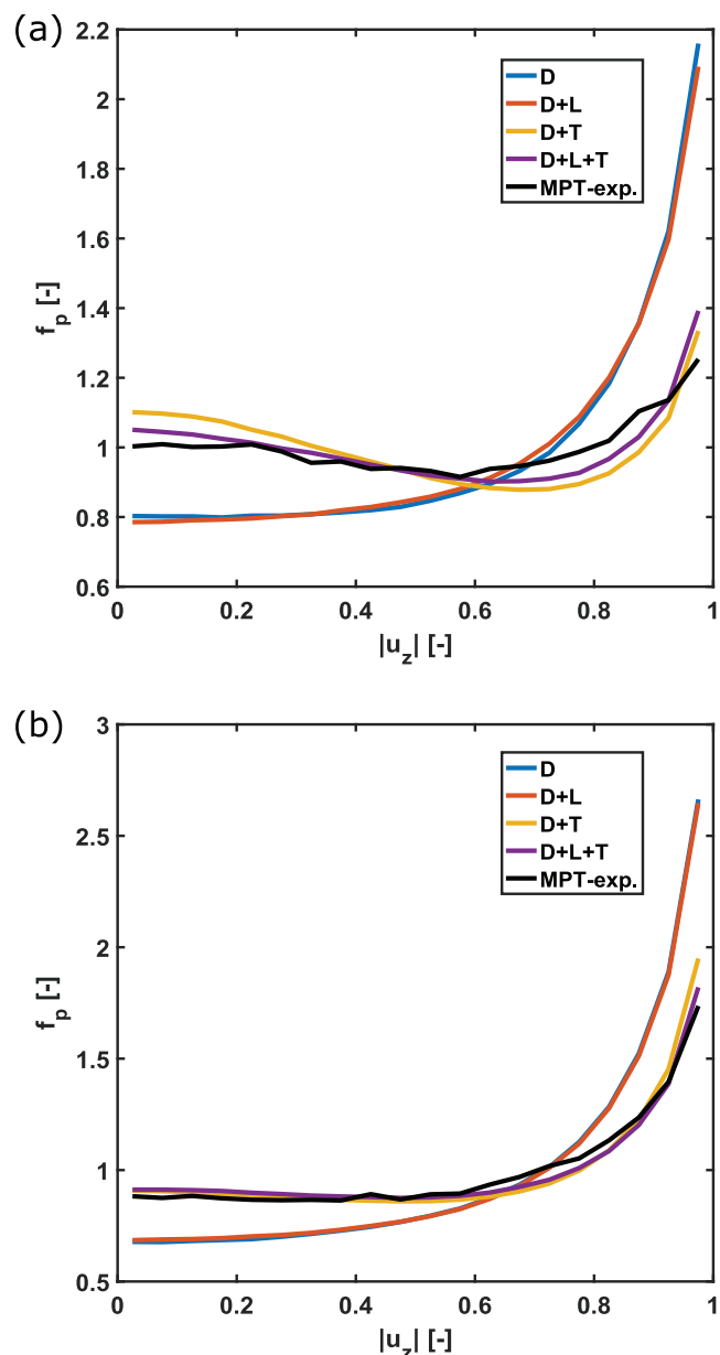
FIGURE 6 Preferred particle orientation at (a) 1.6U_{mf} and (b) 2U_{mf} . Variation of f_p(|u_z|) for simulations with differing hydrodynamic force conditions and from experimental results [Color figure can be viewed at wileyonlinelibrary.com ]
