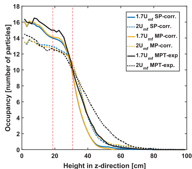
FIGURE 5 Average cell occupancy along the height in z-direction. The dashed red lines indicate the positions along the z-axis used for the sampling of v_z profiles in Section 4.3 [Color figure can be viewed at wileyonlinelibrary.com ]
