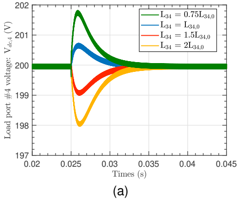
Figure 8: Dynamic behavior of port #4 voltage v_{dc,4} to investigate sensitivity of decoupling performance to deviation in model parameters: (a) CDC decoupling performance when the value of the link inductance L_{34} is changed in the plant model from its nominal value L_{34,0} , and (b) LADRC decoupling performance when the value of the input gain b_4 is changed from its nominal value b_{4,0} .
