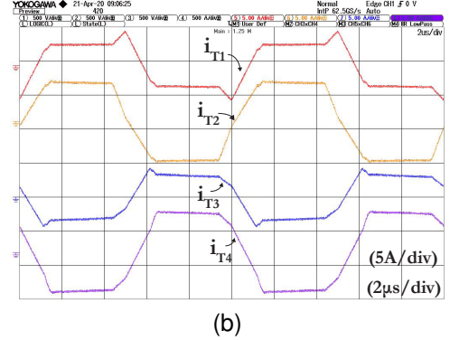
Figure 10: Steady state waveforms of: (a) winding voltages, and (b) winding currents of the QAB converter in 2S-2L mode at operating point: P_{\text{load},4} = -730 \text{ W} ; P_2 = 800 \text{ W} ; P_3 = -400 \text{ W} .
