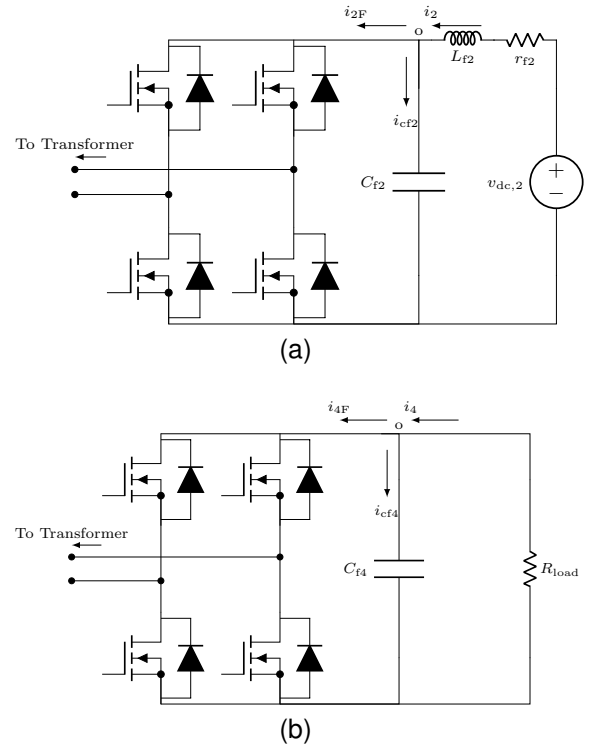
Figure 12: Circuit schematic of QAB converter ports: (a) second order current control port #2 with LC filter, (b) first order voltage control port #4 with only capacitor filter.
