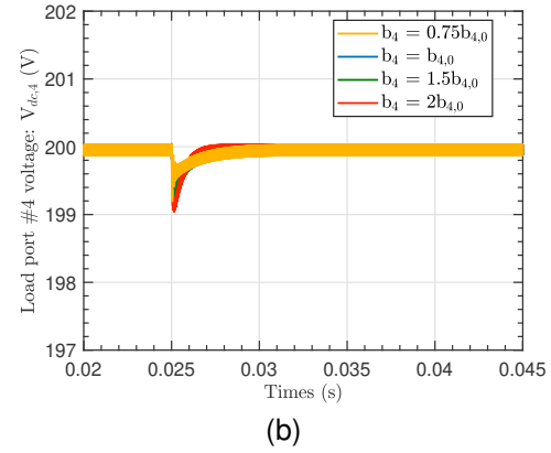
Figure 8: Dynamic behavior of port #4 voltage v_{dc,4} to investigate sensitivity of decoupling performance to deviation in model parameters: (a) CDC decoupling performance when the value of the link inductance L_{34} is changed in the plant model from its nominal value L_{34,0} , and (b) LADRC decoupling performance when the value of the input gain b_4 is changed from its nominal value b_{4,0} .
