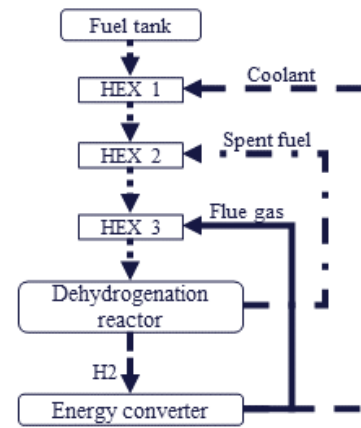
Figure 1: Simplified display of the endothermic model. HEX stands for heat exchanger
