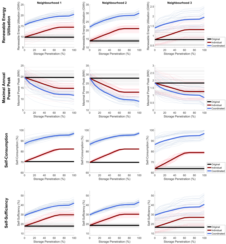
Figure 7.4 Impact of increasing storage penetration and of storage coordination in three neighbourhoods in Amsterdam, the Netherlands. Each panel shows the impact of increasing storage penetration (between 0% and 100% of consumers have their own storage units) for three scenarios: original (without storage, and with individual PVs), individual use of storage and PVs, and coordinated use of storage and PVs. For all plots and scenarios, the PV penetration is kept constant at 50%. The thin lines represent 30 individual simulation runs, the thick lines the averages. Noise is attributed to variations in PV and storage sizes, which result from the random assignment and corresponding sizing of PV and storage systems. Note that in each simulation, the original, individual, and coordinated scenarios are calculated for the same set of PV and storage capacity.
