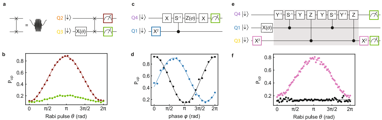
Fig. 3 SWAP, CS -1 and Toffoli-like gate. a A resonant SWAP gate is implemented by applying a Tukey-shaped pulse with an oscillation superimposed to the barrier gate between Q2 and Q3. It is tested using the depicted circuit diagram. b To demonstrate the SWAP gate, a Rabi pulse X(\theta) is applied to Q3, followed by a SWAP gate between Q2 and Q3. Then, either Q2 is read out using readout system Q1Q2 (red) or Q3 is read out using readout system Q3Q4 (green). c Circuit diagram of the experiment demonstrating the CS -1 gate. d The CS -1 gate is obtained by calibrating the phase difference to be -\pi/2 , for the experiments with (blue) and without (black) an X^2 gate on the control qubit Q1. e Circuit diagram of the Toffoli-like gate (gray) composed of CS -1 and CZ gates. f Demonstration of the Toffoli-like gate with target qubit Q4 and control qubits Q1 and Q3. An X(\theta) pulse is applied to Q1 and the final state of Q4 is measured using readout system Q3Q4. Results of the experiment in e with (pink) and without (black) a preparation pulse X^2 on ancilla qubit Q3.
