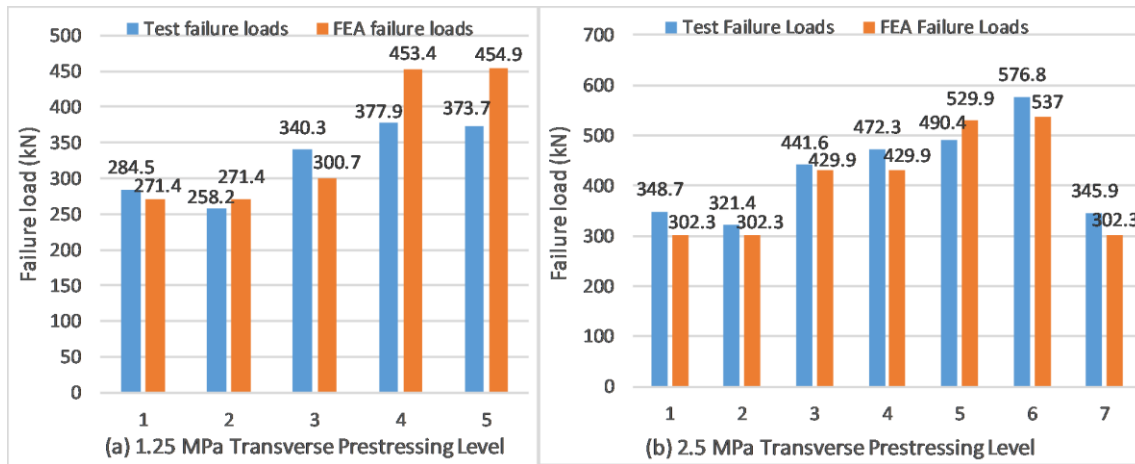
Figure 4. Comparison of the experimental and the finite element analyses failure loads.
