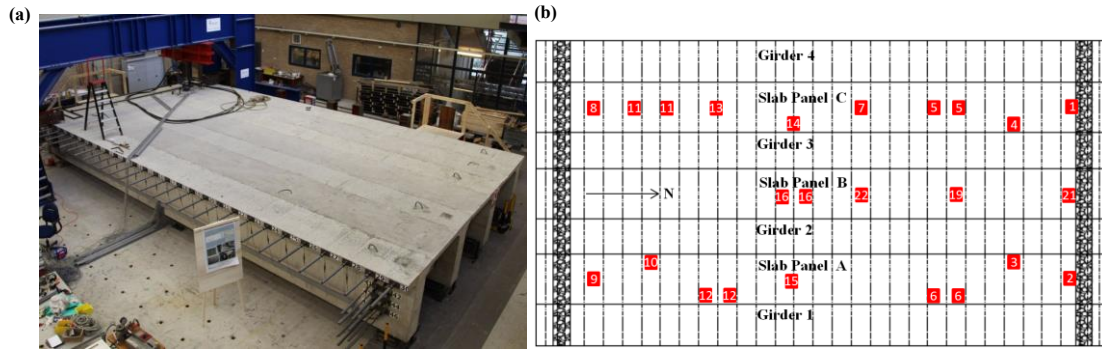
Figure 1. a) Model of the bridge in the laboratory; b) Location of the tests. Prestressing ducts are shown by dashed lines.
