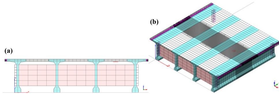
Figure 5. The FE real bridge model for P1M load case: a) Cross-section; b) 3D view.
