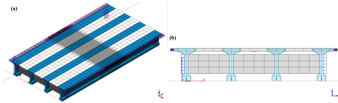
Figure 3. a) 3D finite element model simulating the lab prototype; b) Transverse section of the model.
