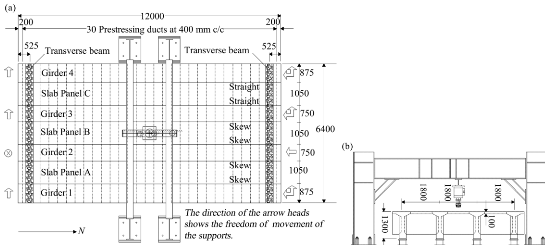
Figure 2. Experimental setup: a) Top view b) Transverse view. Shown dimensions are in mm.
