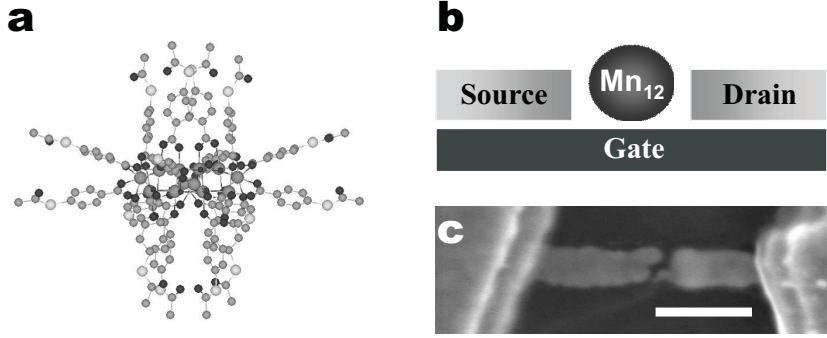
Figure 6.1: a , Side view of a Mn 12 molecule with tailor made ligands containing acetyl-protected thiol end groups (R=C 6 H 4 ). Atoms are color labelled: Manganese (gray, large), oxygen (dark gray), carbon (gray), sulfur (light gray). The diameter of the molecule is about 3 nm. b , Schematic drawing of the Mn 12 molecule (circle) trapped between electrodes. A gate changes the electrostatic potential on the molecule enabling energy spectroscopy. c , Scanning electron microscopy image of the electrodes. The gap is not resolvable. Scale-bar corresponds to 200 nm.
