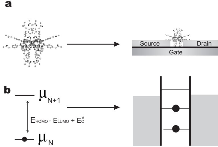
Figure 2.5: When a single molecule (a) is weakly contacted by metallic leads it behaves as a quantum dot. b, The electronic structure of the isolated molecule is ‘compressed’ due to screening by the leads.
