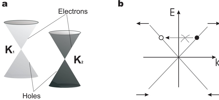
Figure 2.14: Small k approximation. a , The conical approximation of the band structure around the two inequivalent K -points. In the absence of intervalley scattering, the two subbands or valleys are independent. b , Projection of one of the two cones on an arbitrary k - E plane. The arrows denote the pseudo spin which is always aligned (anti-aligned) to \mathbf{k} for electrons (holes). Scatter processes that do not conserve pseudo-spin are not allowed (dashed arrow).
