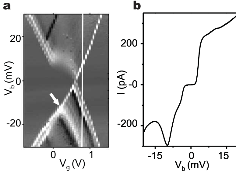
Figure 6.3: a , Differential conductance (grayscale) as a function of gate voltage ( V_g ) and bias voltage ( V_b ) for another device ( T = 1.5 K, R=\text{C}_6\text{H}_4 ) in which the 2 meV and 3 meV excitations are also observed (negative bias). The 14 meV excitation is indicated by a white arrow. The origin of the step in the diamond edge at positive bias is unclear, but most likely not related to the magnetic properties of the molecule. (gray-scale from -3 nS [black] to 10 nS [white]) b , I - V_b along the line in (a).
