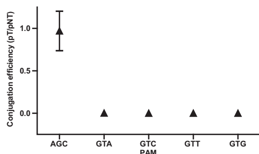
Figure 3. Conjugation Efficiency of Target Plasmids Carrying either AGC-Protospacer1 or GTN-Protospacer1 in Synechocystis 6803
