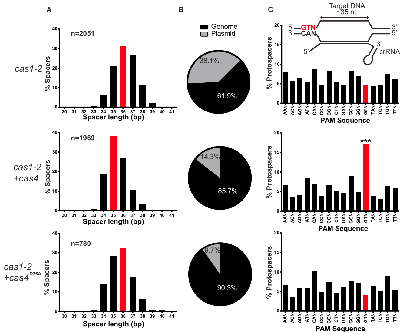
Figure 2. Analysis of Spacers Acquired by Type I-D CRISPR Adaptation
