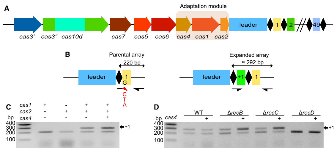
Figure 1. Genetic Requirements of Type I-D CRISPR Adaptation
