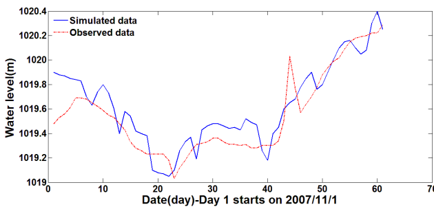
Fig. 4. Verification of the model: water levels.
