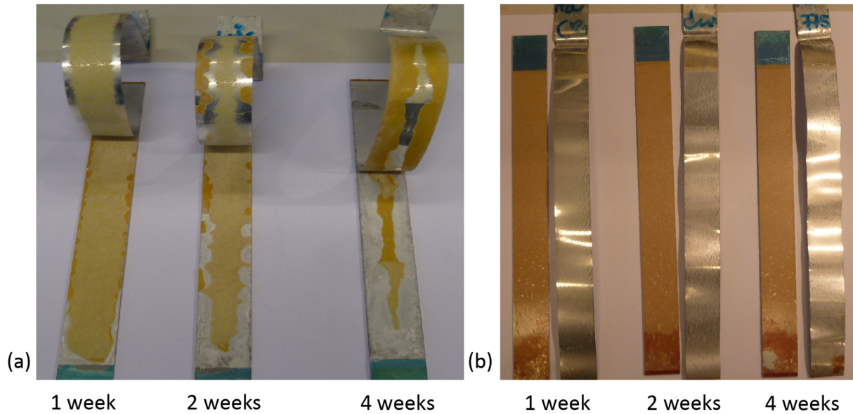
Figure 10: Macroscopic images of the peeled panels after various periods in the salt spray cabinet. Panels received hydrothermal pre-treatment with FM 73 (a) and Redux 775 adhesives (b), without any primer.
