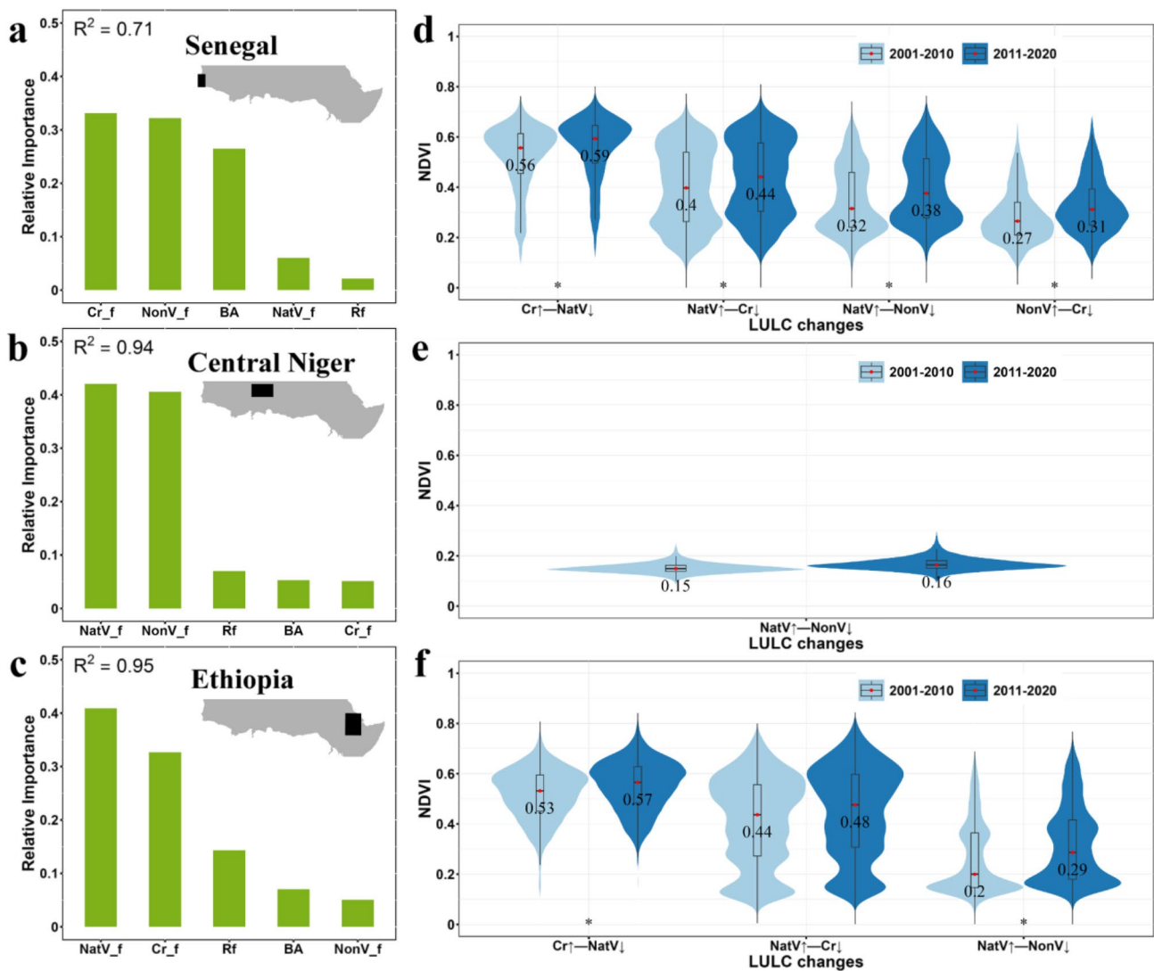
Fig. 6 a–c The relative importance of rainfall variation (Rf), change in cropland fraction (Cr f ), change in natural vegetation fraction (NatV f ), change in non-vegetation fraction (NonV f ), and change in burned area (BA) to the NDVI anomalies (Z-score of NDVI) within non-rainfall-driven greening clusters in the Sudano-Sahelian region during 2001–2020. R^2 in the figures is the coefficient of determination of the multiple linear regression between the Z-score of NDVI and
