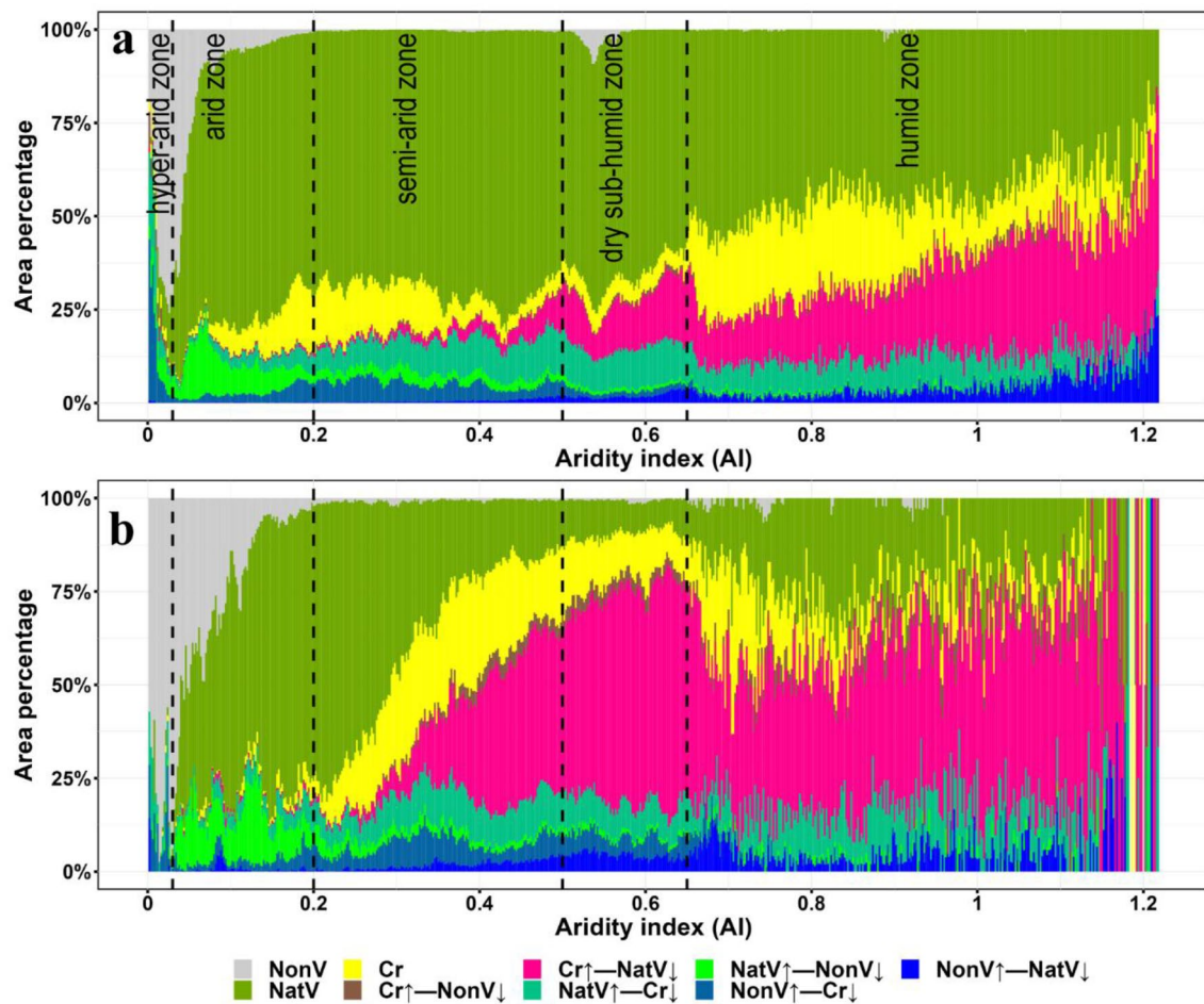
Fig. 4 Fractional abundance of LULC change types contributing to a greening and b browning vs. aridity index (AI); the bin width of AI values (x-axis) was set to 0.002. The vertical dashed lines indicate the climate zones divisions used in this paper. For the
