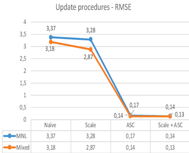
Fig. 7. RMSE measure.
