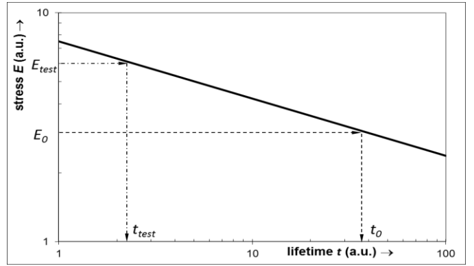
Fig. 2. Example of a power law relationship of (3). Enhancing the rated stress E_0 to the test stress E_{\text{test}} accelerates the time to breakdown from t_0 to t_{\text{test}} .
