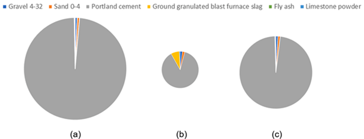
Fig. 1. Global warming potential of concrete based on raw material composition as indicated in Table 1 with (a) CEM I concrete (2.93E+02 kg CO 2 eq/m 3 concrete), (b) CEM III/B concrete (9.85E+01 kg CO 2 eq/m 3 concrete) and (c) CEM II/B-V concrete (2.07E+02 kg CO 2 eq/m 3 concrete). For these three specific mix designs, CEM I concrete contributes respectively 1.4 and 3.0 times more to the global warming potential compared to CEM II/B-V and CEM III/B concrete.
