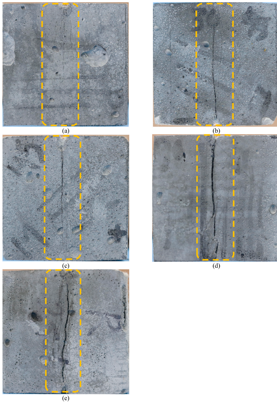
Fig. 11. Splitting strength of specimen at different fiber angle: (a) SC-0; (b) SC-30; (c) SC-45; (d) SC-90 and the (e) S-R specimens.
