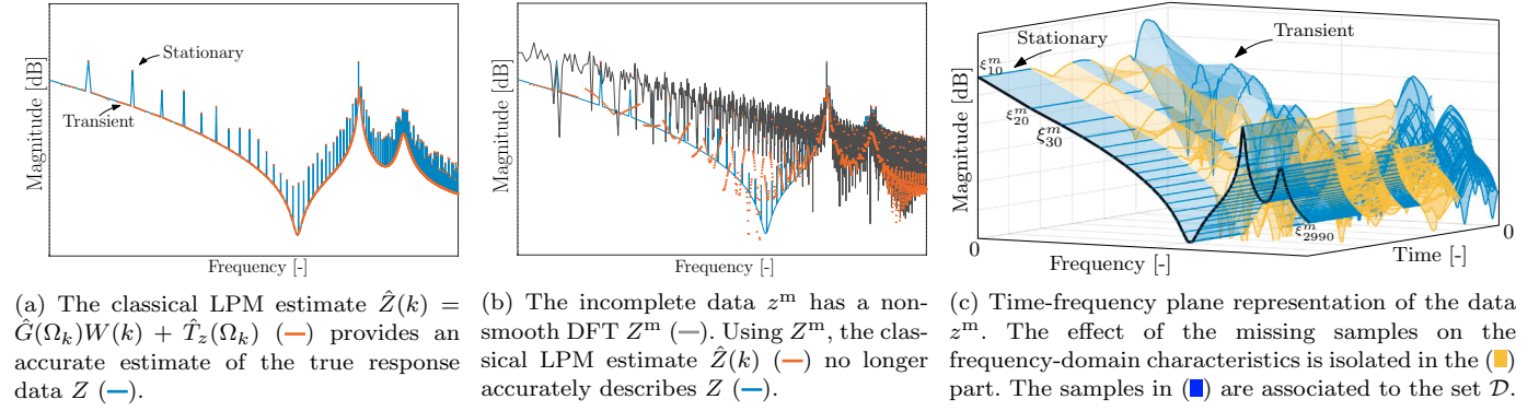
Fig. 2. Example of LPM estimation of Z(k) = G(\Omega_k)W(k) + T_z(\Omega_k) with and without missing samples.
