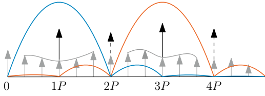
Fig. 4. Frequency-domain representation of Z in (1) for P = 3, \gamma = 1 without noise. At the EF lines [1P, 2P, 3P, 4P] , the response consists of the transient (grey arrows) and periodic response (black arrows). At the remaining NEF lines, the response contains only transient contributions. The grey curves represent the local transient estimates based on the n_r lines around the [1P, 3P] odd EF lines. The frequency-domain weights introduced by \Psi_{1P} and \Psi_{3P} are shown in (—) and (—).
