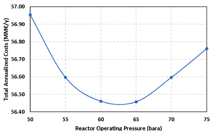
Fig. 6. Total annualized costs (TAC) at various reactor pressures.
