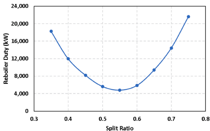
Fig. 12. Reboiler duty vs liquid split ratio for the DWC.
