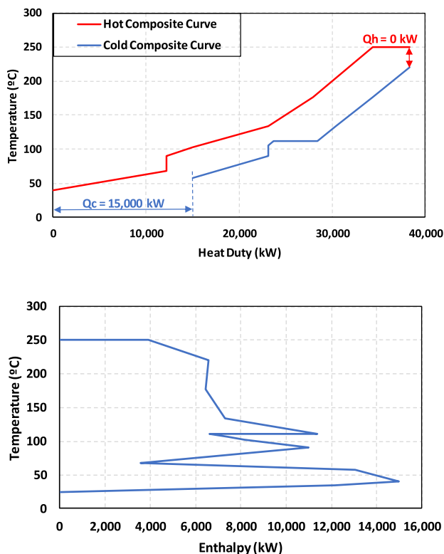
Fig. 2. Hot and cold composite curves (upper graph) and Grand Composite Curve (lower graph) of a thermally self-sufficient process for methanol production by CO 2 hydrogenation.
