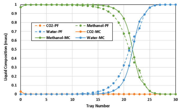
Fig. 13. Composition profiles along the DWC.
