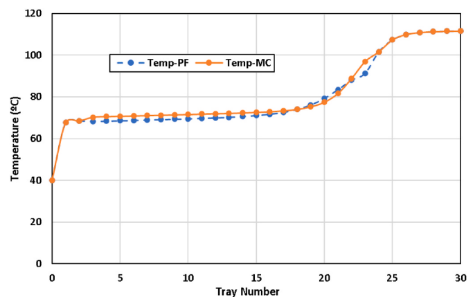
Fig. 14. Temperature profiles along the DWC.
