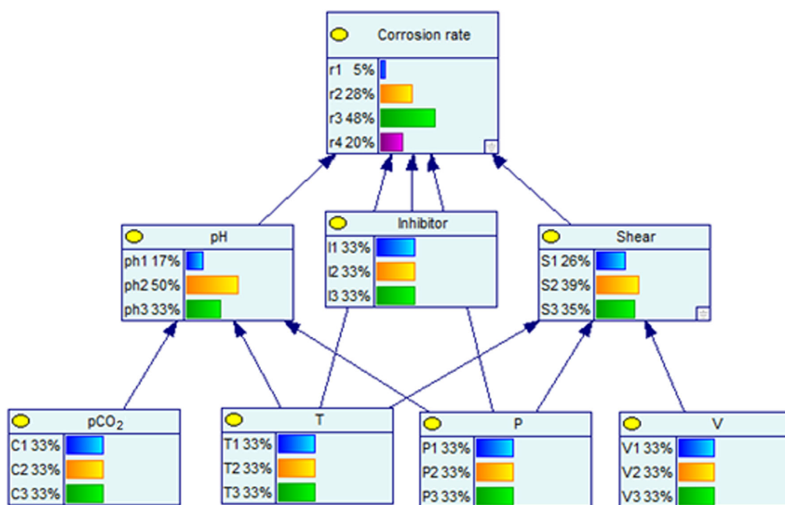
FIGURE 3 BN developed for predicting CO 2 corrosion rate
