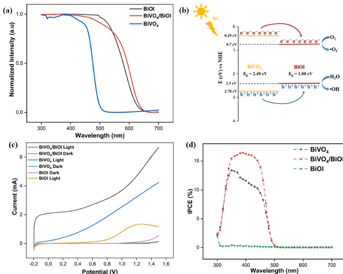
Fig. 5. (a) UV–Visible diffusive reflectance spectra of BiVO 4 , BiOI and BiVO 4 /BiOI photoanodes showing the absorbance range (b) Illustration of photogenerated holes and electrons for the generation of •OH and •O 2 - radicals after the interaction of solar photons with BiVO 4 /BiOI photoanode (c) LSV curves for BiVO 4 , BiOI and BiVO 4 /BiOI photoanodes under dark and illuminated conditions performed from −0.2 to 1.5 V at 100 mV s −1 scan rate (d) IPCE plots for BiVO 4 , BiOI and BiVO 4 /BiOI photoanodes under 1 sun illumination at 1 V external bias vs platinum wire as counter electrode.
