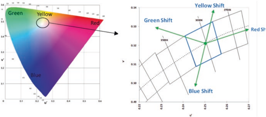
Fig. 8.10 Illustration of color shifts in the CIE 1976 color space. Any change in the spectral proportion of any colors results in a chromaticity shift [14, Reproduced with permission]
