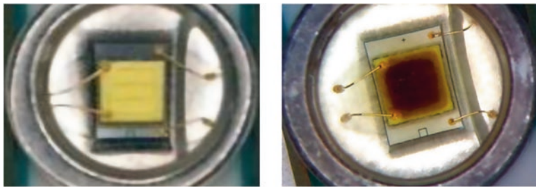
Fig. 8.3 Influence of thermal aging on the discoloration of LED optical package [47, Reproduced with permission from authors]
