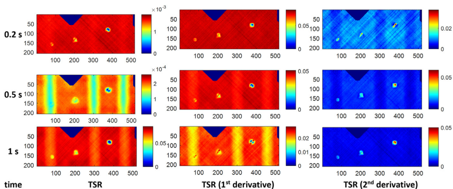
Figure 8.9 Results of TSR and its first and second derivatives for the second CFRP sample at various times.
