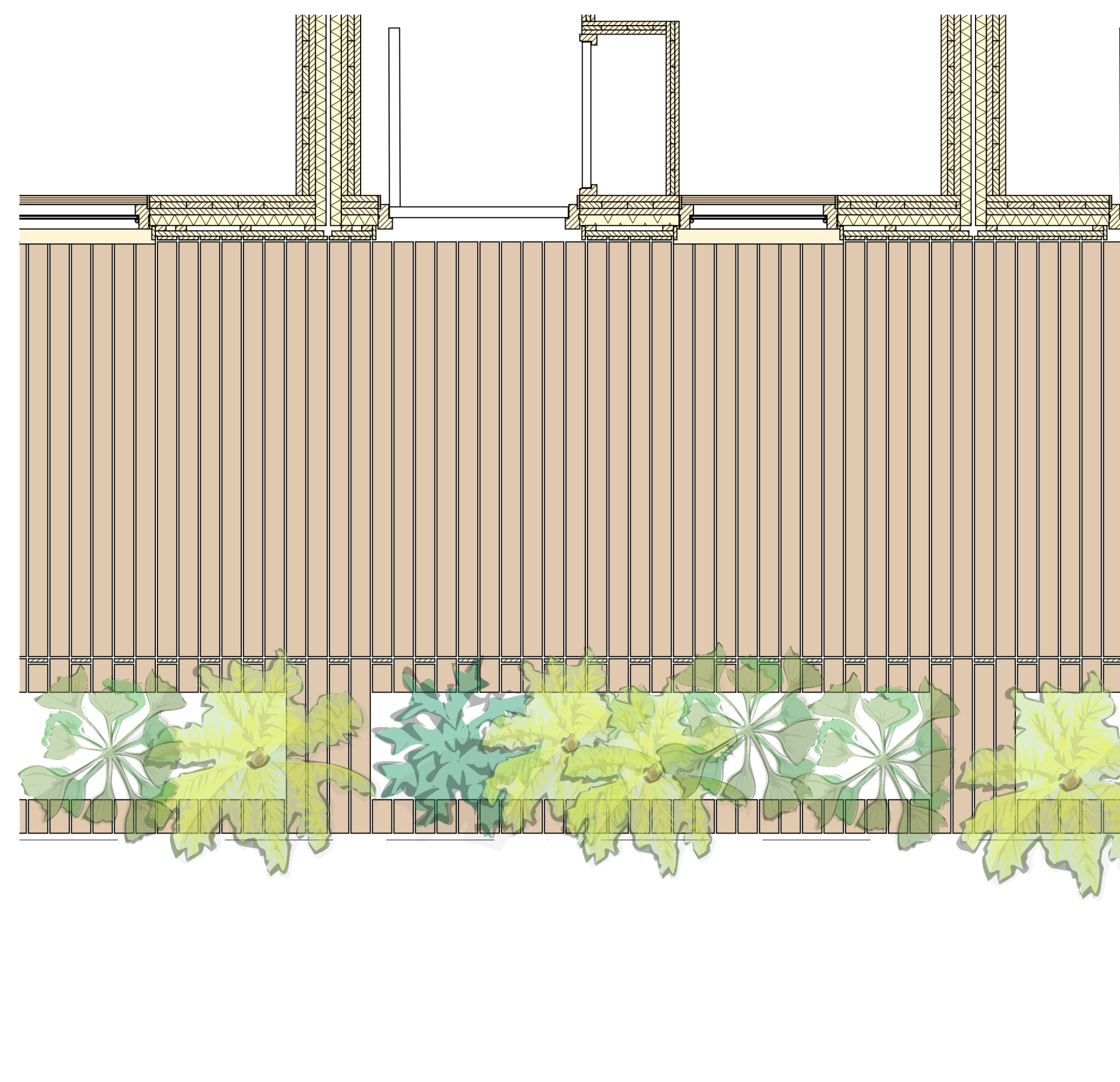
D-04 Horizontal Section Gallery Facade 1:20
