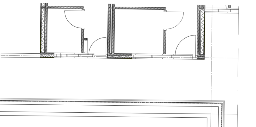
D-15 Horizontal Section Street 1:50
