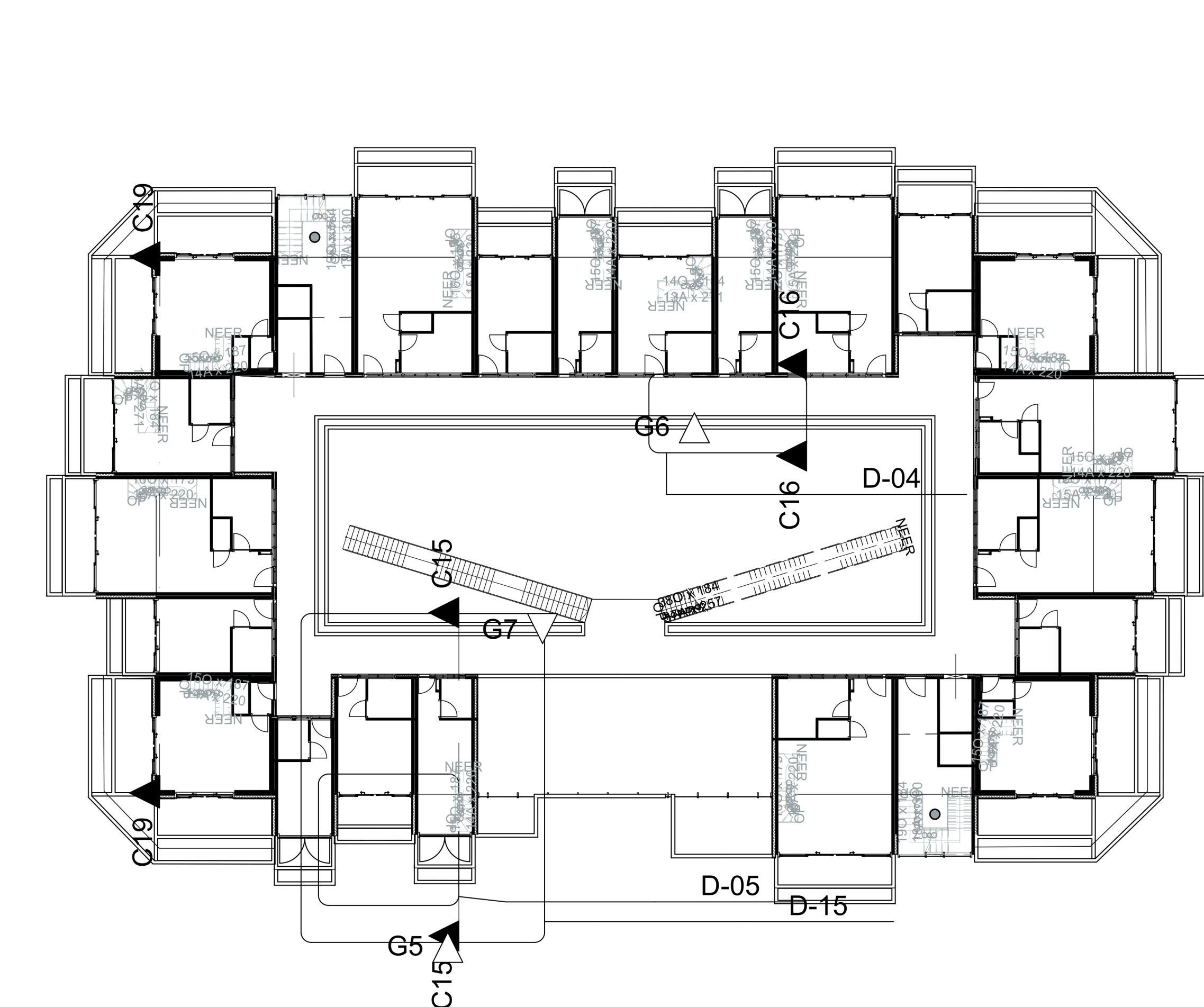
9. Basic Floorplan 1:200
