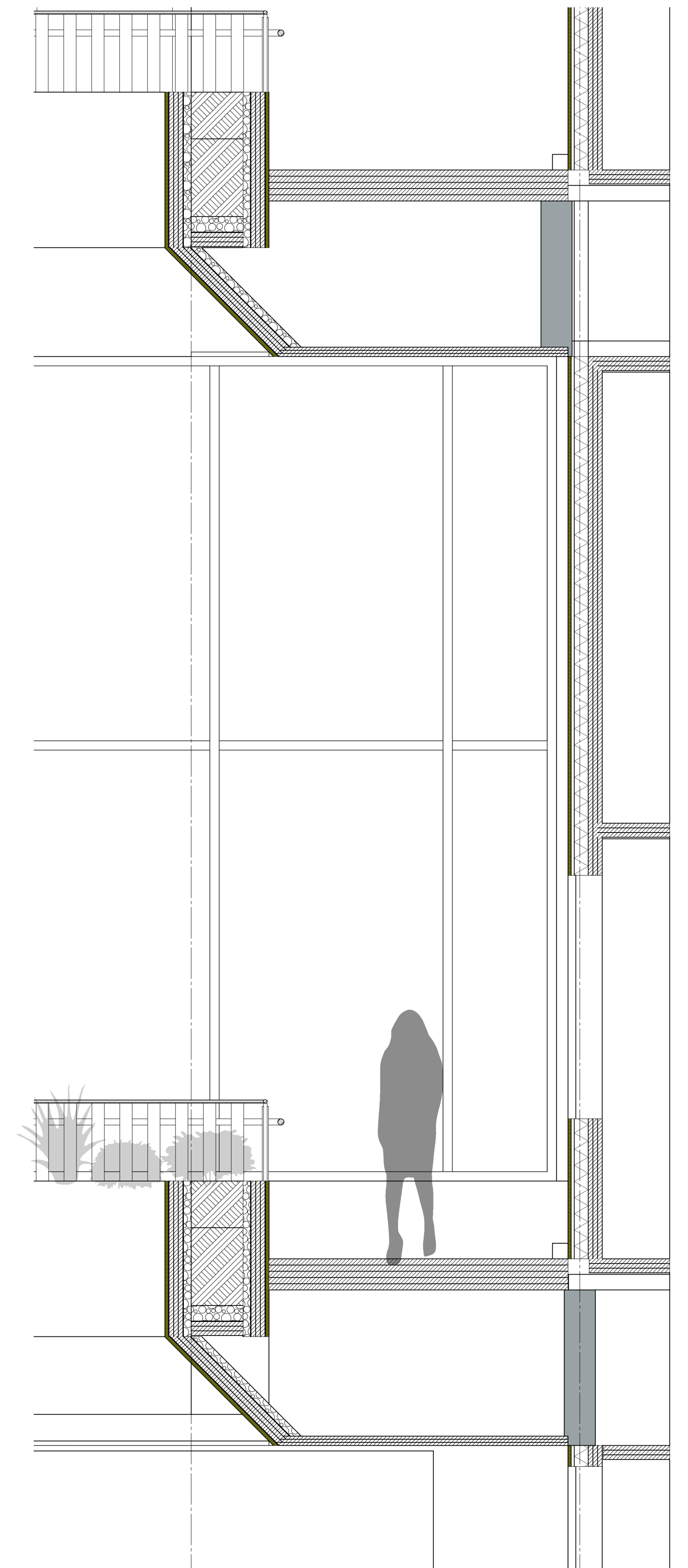
C16 Section Gallery Facade 1:20
