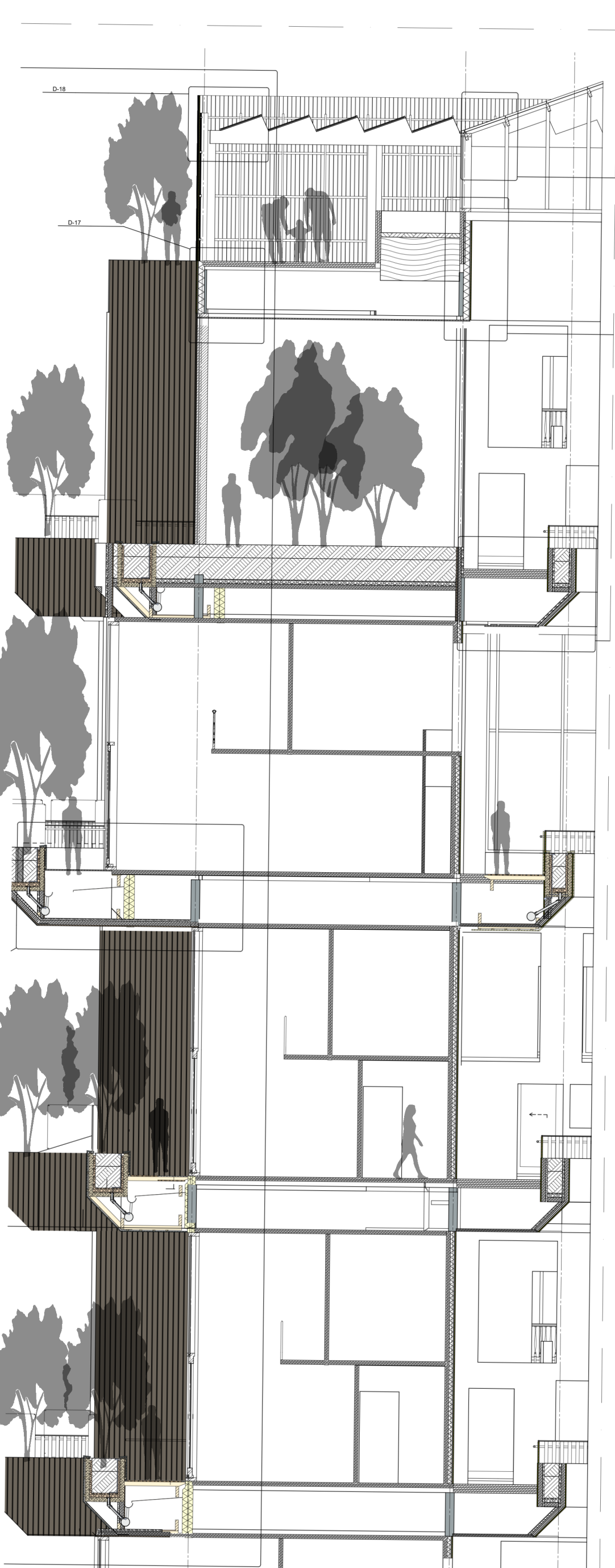
D-12 Section South Side 1:50
