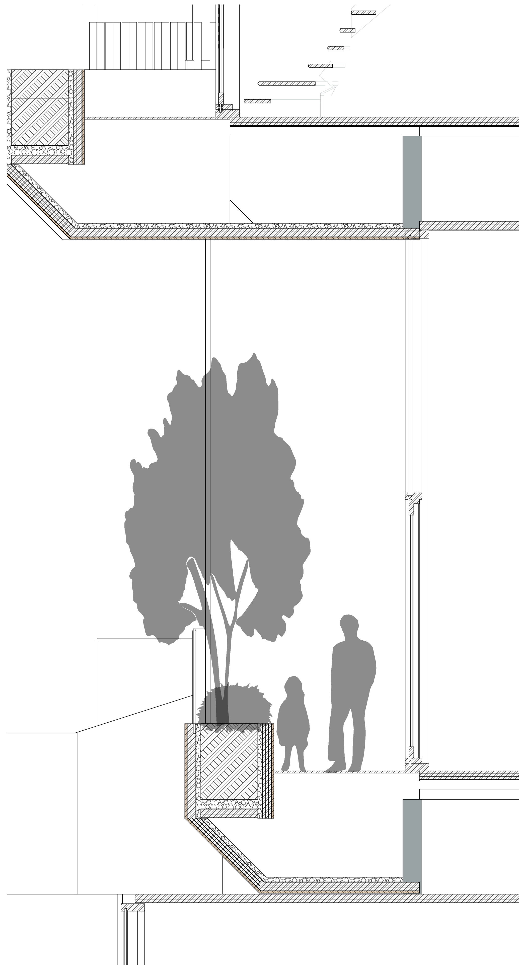
C15 Section South Facade 1:20
