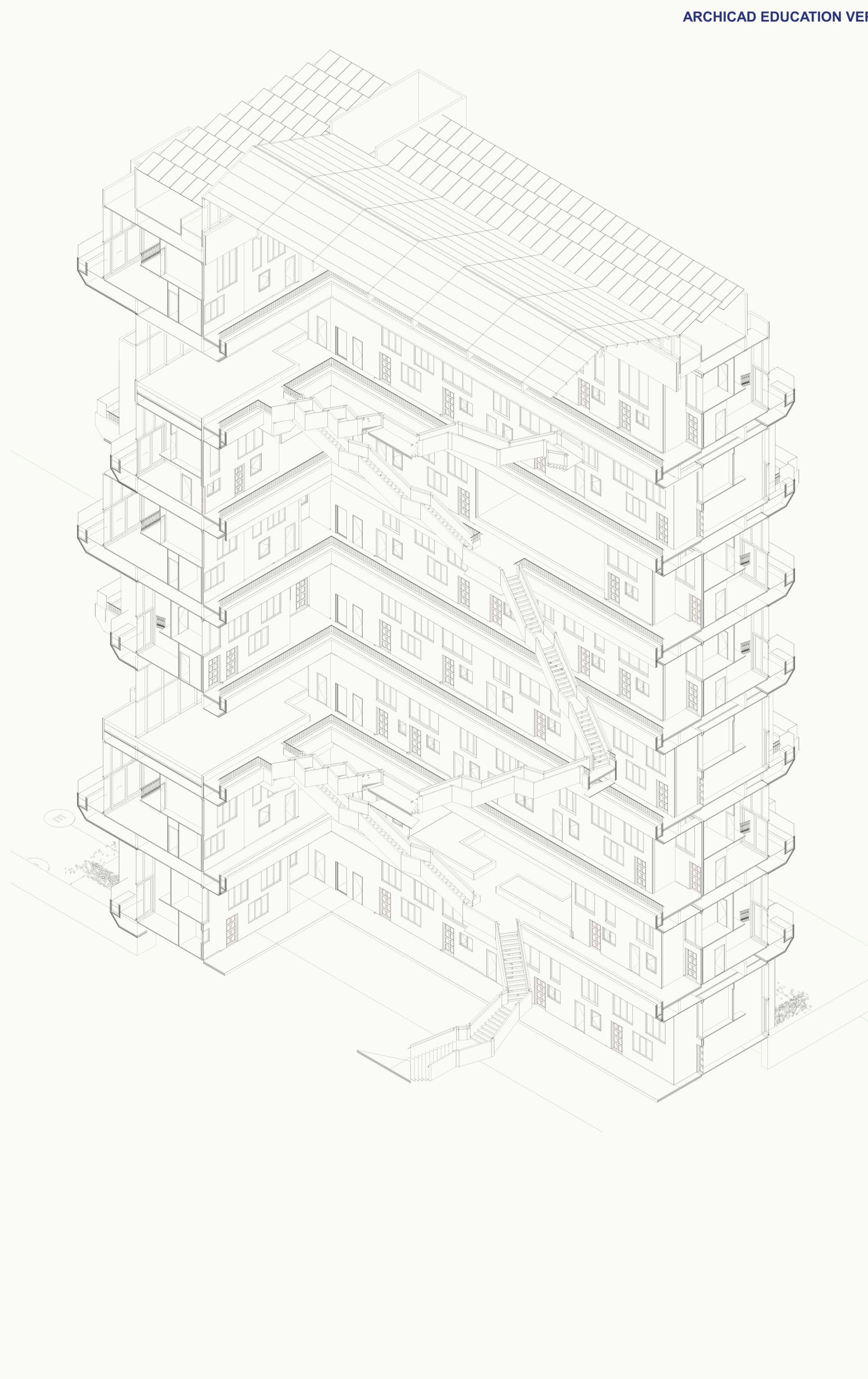
Generic Axonometry
