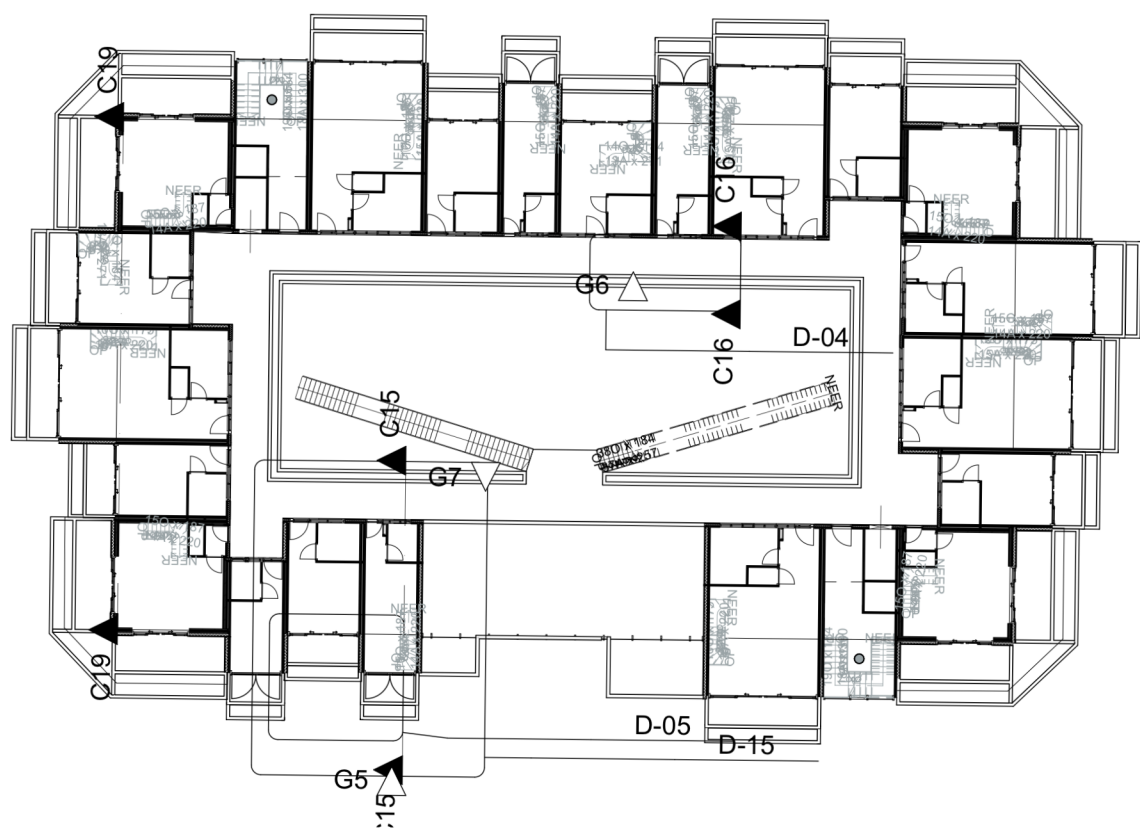
Basic Floorplan 1:200
