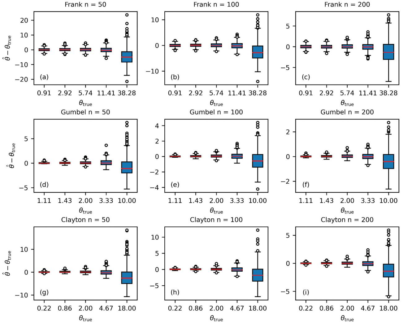
Figure 4. Box plots of (\hat{\theta} - \theta_{true}) for different copulas and different sample sizes.
