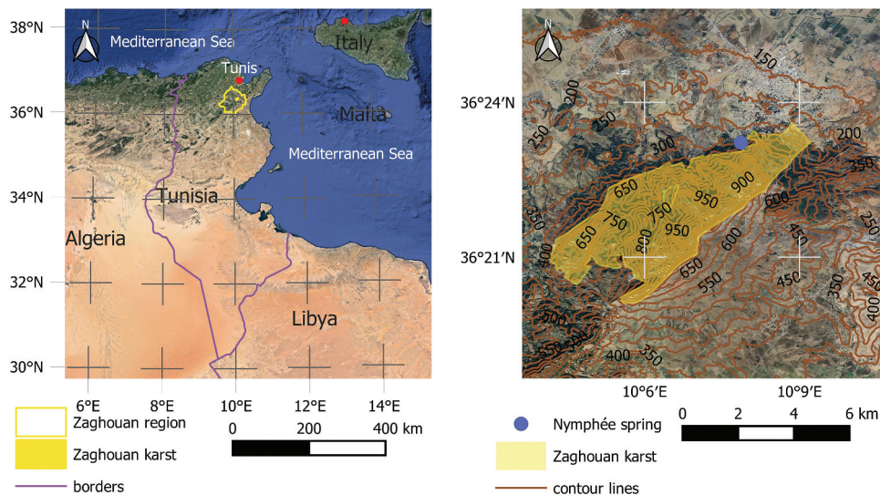
Figure 11. Location of the karst area. Both figures combine Google Map data ©2015 with material from Natural Earth.
