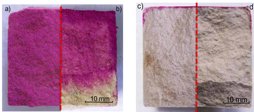
FIGURE 5.9 Pictures of the phenolphthalein test performed on the cross sections of specimens of Maastricht limestone treated with (a) E25 and (b) B25 and of Migné limestone treated with (c) E25 and d) B25. The absorption surface is on the top of the figures.
