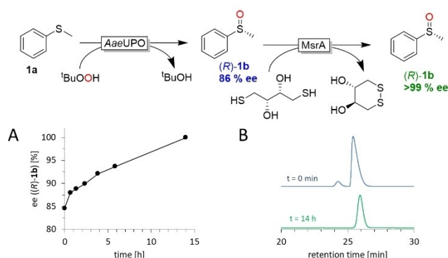
Figure 4. Polishing the optical purity of (R)-1b by MrsA-catalysed stereoselective reduction of the contaminating (S)-enantiomer. (A) Time course (B) corresponding HPLC chromatograms. Reaction conditions: [(R)-1b, 85% ee] = 15 mM (2 g), [MrsA] = 25 μM (9.4 mL), [DTT] = 56 mM (8.214 g), acetonitrile = [2% v/v, 19 mL], PBS buffer (50 mM, pH 6.5), total 944 mL, 35 °C, 800 rpm, 14 h.
