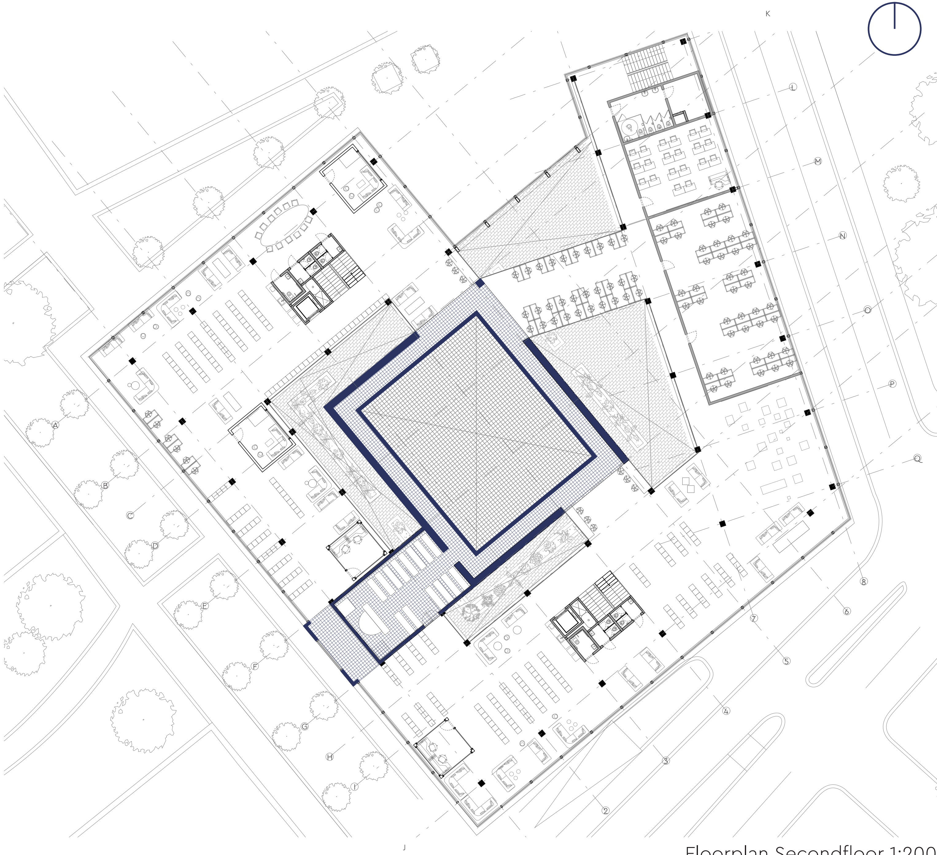
Floorplan Secondfloor 1:200
