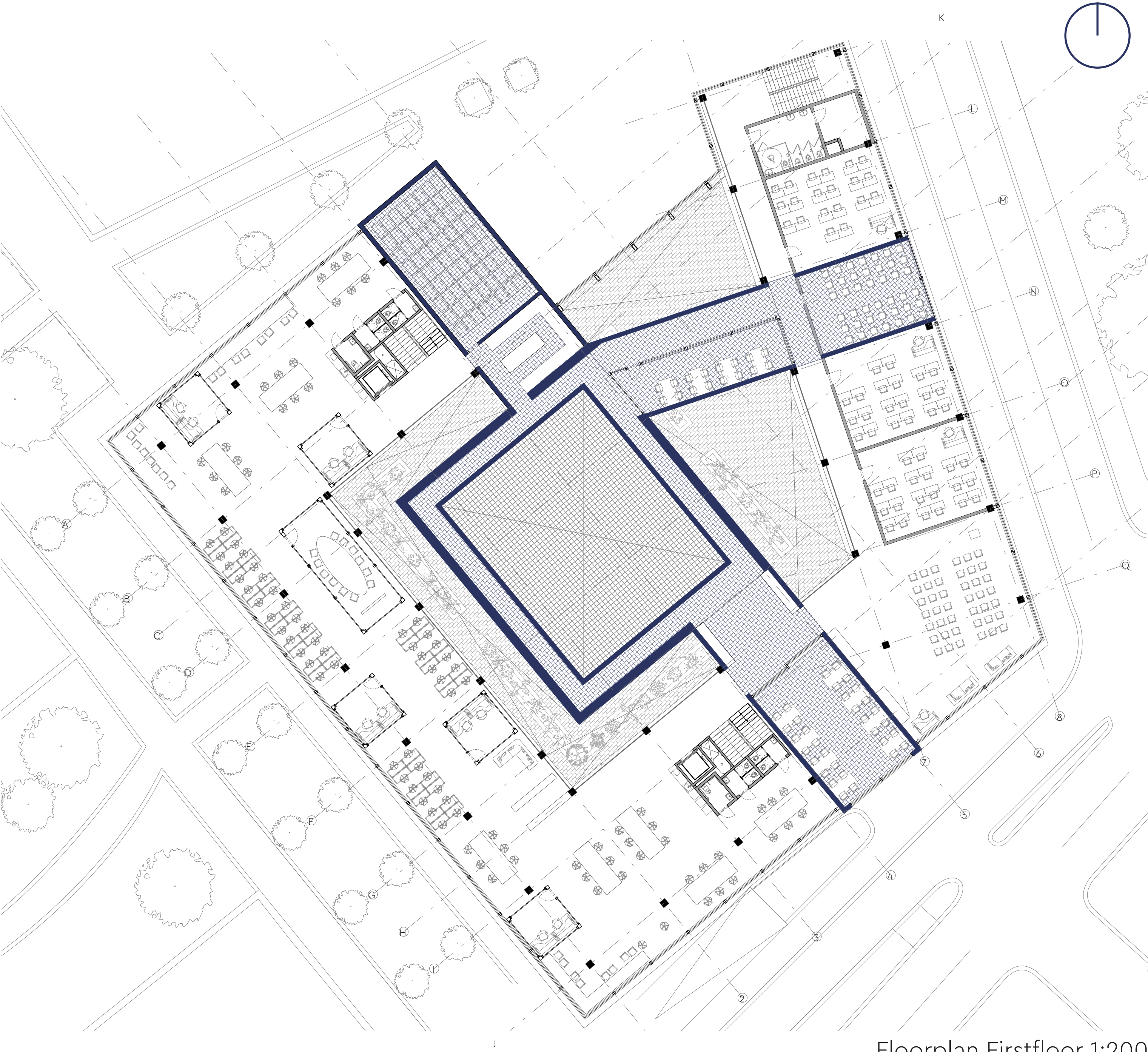
Floorplan Firstfloor 1:200
