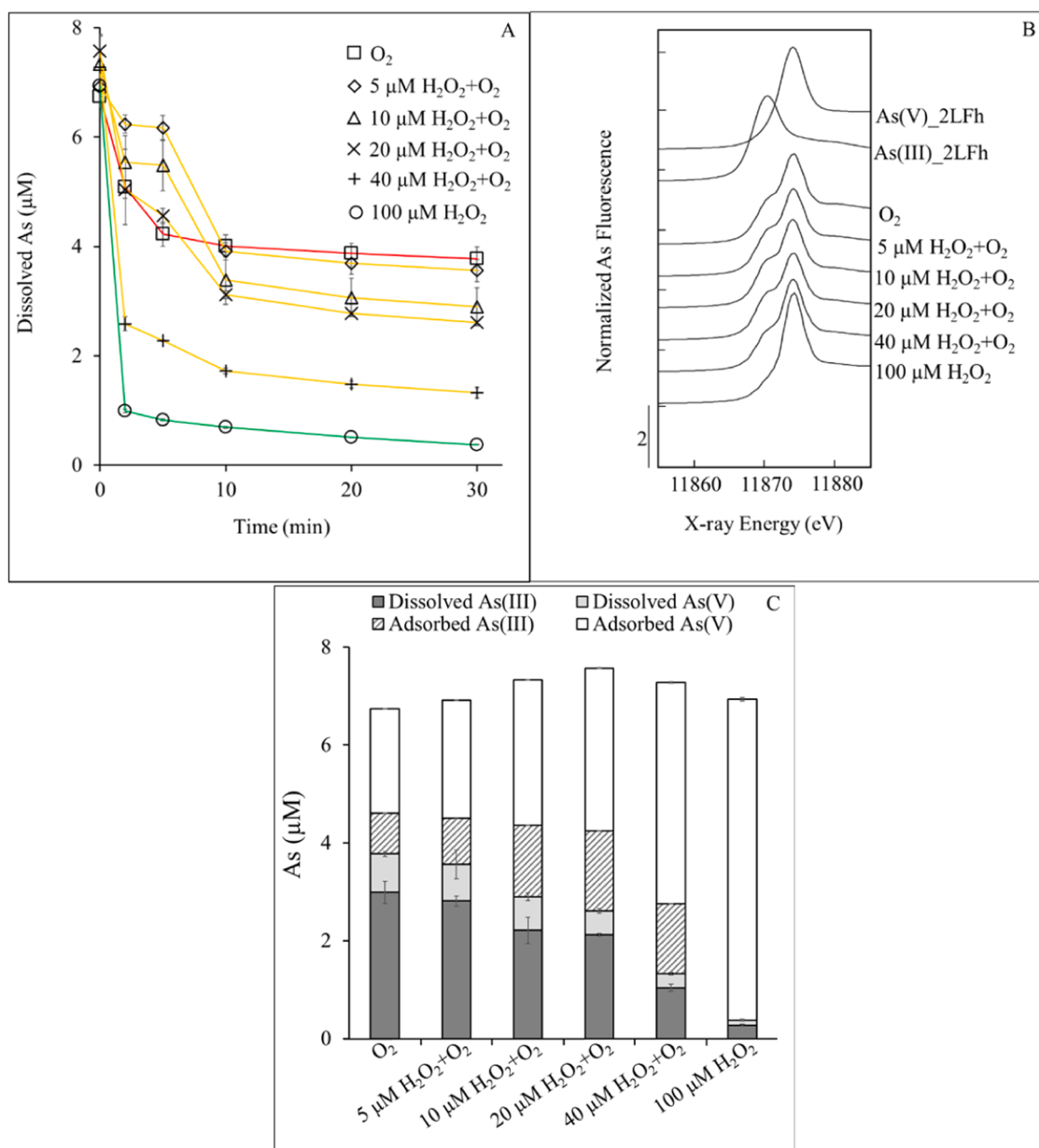
Fig. 2. Removal of initial As(III) over 30 min (A), As K-edge XANES spectra of the generated Fe solids (B), and As speciation at the experiment end (t = 30 min) when 100 \pm 3 \mu\text{M} Fe(II) was oxidized by 8.0–9.0 mg/L \text{O}_2 (aerobically; t = 0–30 min) (red line), 100 \mu\text{M} \text{H}_2\text{O}_2 (anaerobically; t = 0–30 min) (green line), or sequentially by 5, 10, 20, or 40 \mu\text{M} \text{H}_2\text{O}_2 (anaerobically; t = 0–5 min) followed by 8.0–9.0 mg/L \text{O}_2 (aerobically; t = 5–30 min) (yellow line). Solutions initially contained 7 \pm 0.5 \mu\text{M} As(III), 2.5 mM \text{NaHCO}_3 , and 10 mM NaCl. Data points and error bars represent the average and standard deviation of the samples obtained from replicate experiments.
