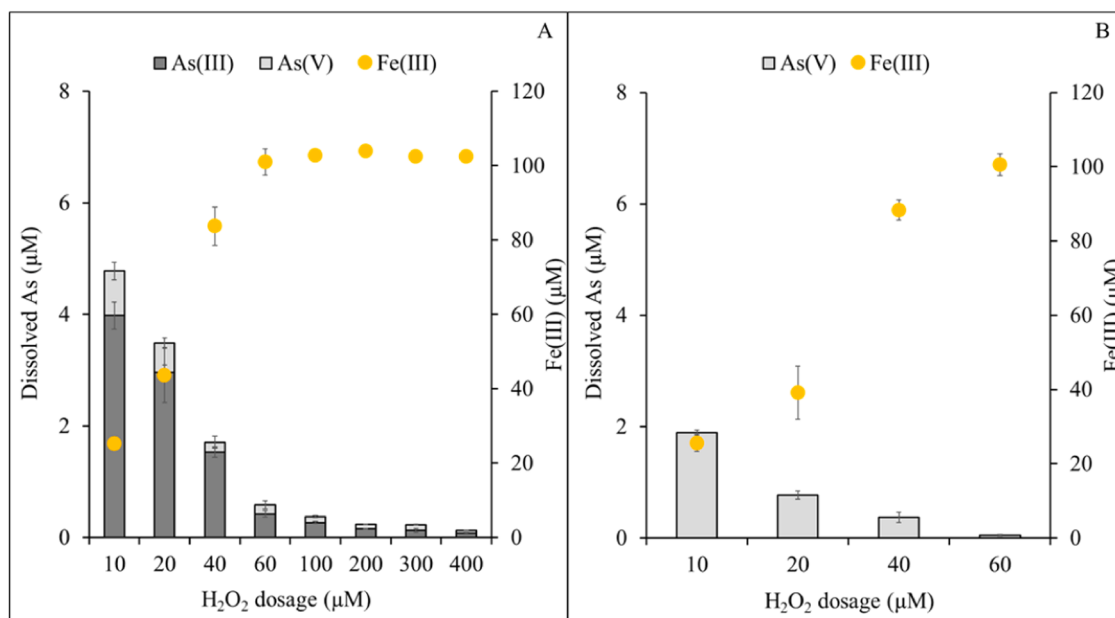
Fig. 3. Dissolved As and Fe(III) concentration in solutions at t = 30 min plotted as a function of different \text{H}_2\text{O}_2 dosage when 100 \pm 3 \mu\text{M} of Fe(II) was oxidized by 10–400 \mu\text{M} \text{H}_2\text{O}_2 anaerobically. Solutions initially contained 7 \pm 0.2 \mu\text{M} As(III) (A) or 7 \pm 0.5 \mu\text{M} As(V) (B), 2.5 mM \text{NaHCO}_3 , and 10 mM \text{NaCl} . All Fe(III) formed solids and no dissolved Fe(III) was measured (data not shown). Data points and error bars represent the average and standard deviation of the samples obtained from replicate experiments.
