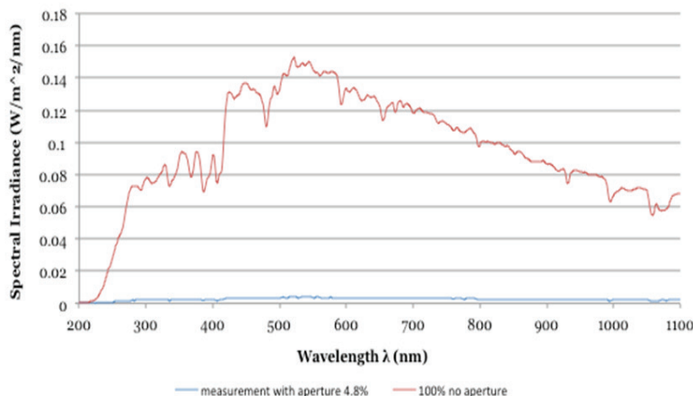
FIGURE 4.20: SPECTRAL IRRADIANCE ( \text{W}/\text{m}^2/\text{nm} ) MEASURED AT DISTANCE 2 CM FROM THE WINDOW AT A SOUTH ORIENTED OFFICE AT DELFT, THE NETHERLANDS, ON JUNE 10TH, 2015.
