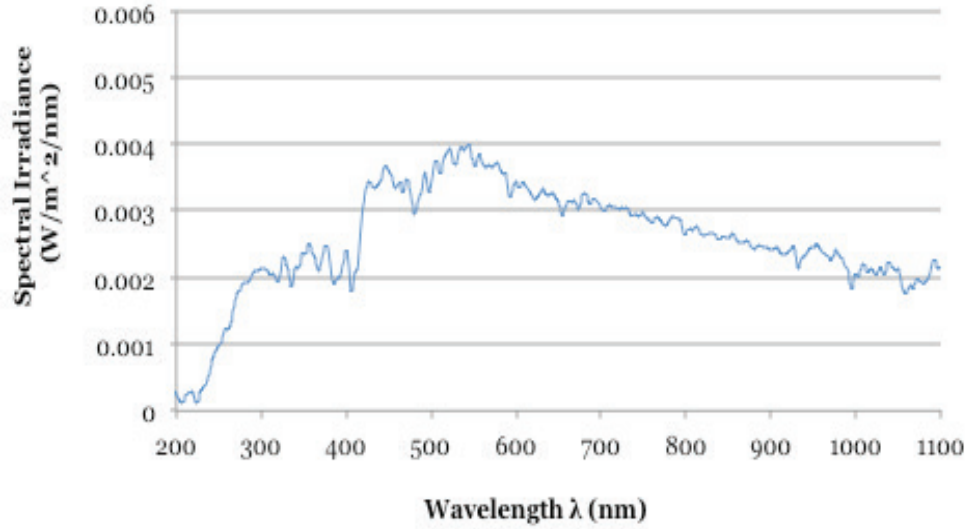
FIGURE C1.7: SPECTRAL IRRADIANCE ( \text{W/m}^2/\text{nm} ) MEASURED AT DISTANCE 2 CM FROM THE WINDOW AT A SOUTH ORIENTED OFFICE AT DELFT, THE NETHERLANDS, ON JUNE 10TH, 2015. WINDOW IS OPEN DURING THE MEASUREMENTS AND LIGHTS ARE ON. FOR THESE MEASUREMENTS AN APERTURE WAS USED, WHICH ALLOWS AROUND 4.8 % OF THE LIGHT TO PASS THROUGH THE COVER.
