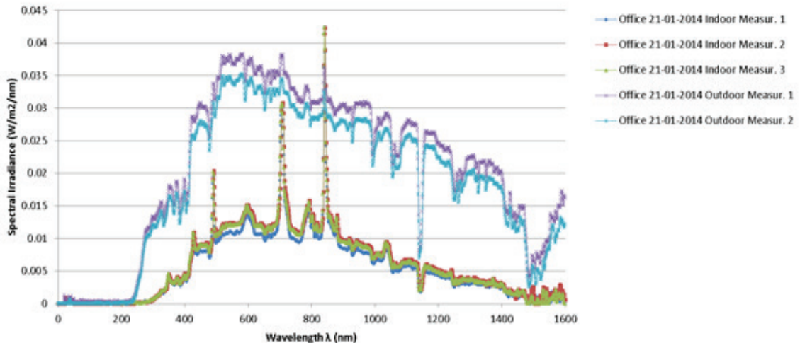
FIGURE C2.1: SPECTRAL IRRADIANCE MEASUREMENTS ( \text{W/m}^2/\text{nm} ) ON 21.01.2014, AT A NORTH ORIENTED OFFICE AT TU DELFT.
