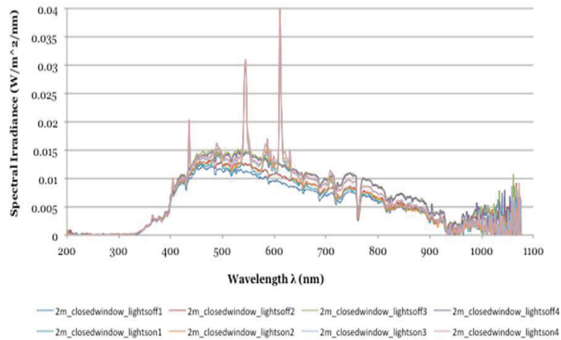
FIGURE 4.14: SPECTRAL IRRADIANCE ( \text{W/m}^2/\text{nm} ) MEASURED AT DISTANCE 2 M FROM THE WINDOW AT A NORTH ORIENTED OFFICE AT DELFT IN THE NETHERLANDS ON JUNE 10TH 2015. THE WINDOW IS CLOSED DURING THE MEASUREMENTS AND THE LIGHTS ARE ON AND OFF RESPECTIVELY.
