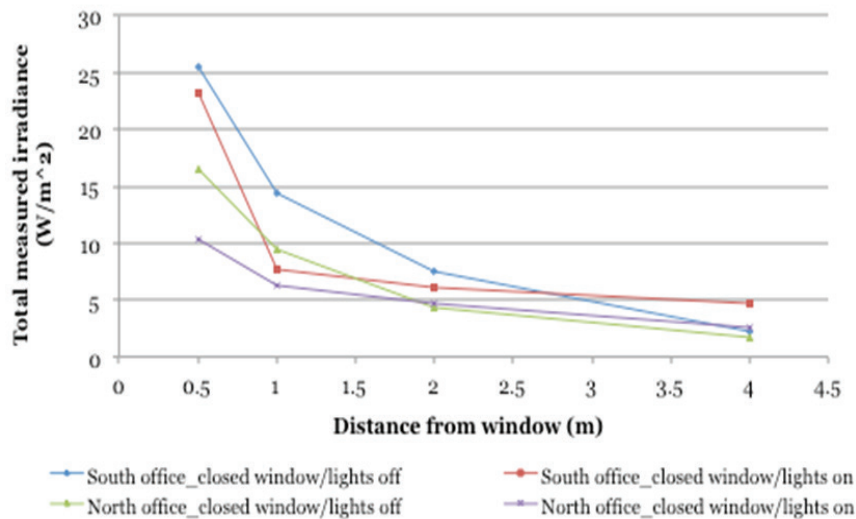
FIGURE 4.21: TOTAL MEASURED IRRADIANCE ( \text{W/m}^2 ) AT A NORTH- AND A SOUTH-FACING OFFICE ON JUNE 10TH, 2015, AT DELFT, THE NETHERLANDS. IN BOTH CASES THE WINDOW WAS CLOSED DURING THE MEASUREMENTS, WHILE THE LIGHTS WERE ON FOR THE RED AND THE PURPLE LINE AND OFF FOR THE BLUE AND THE GREEN.
