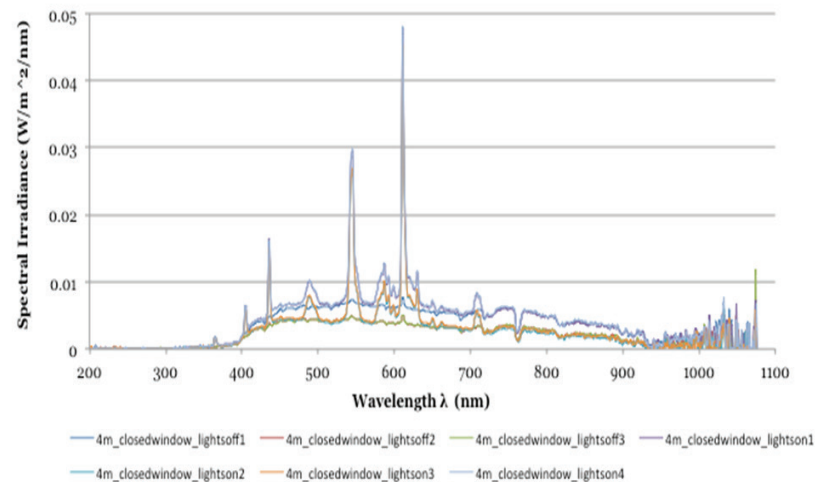
FIGURE 4.15: SPECTRAL IRRADIANCE ( \text{W/m}^2/\text{nm} ) MEASURED AT DISTANCE 4 M FROM THE WINDOW AT A NORTH ORIENTED OFFICE AT DELFT, THE NETHERLANDS, ON JUNE 10TH, 2015. THE WINDOW WAS CLOSED DURING THE MEASUREMENTS AND THE LIGHTS WERE ON AND OFF RESPECTIVELY.
