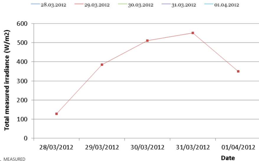
FIGURE 4.25: TOTAL MEASURED IRRADIANCE (W/m 2 ) AT A NORTH FACING OFFICE, SENSOR'S POSITION N1, DELFT 28.03.2012 TO 01.04.2012 AT 12:00.
