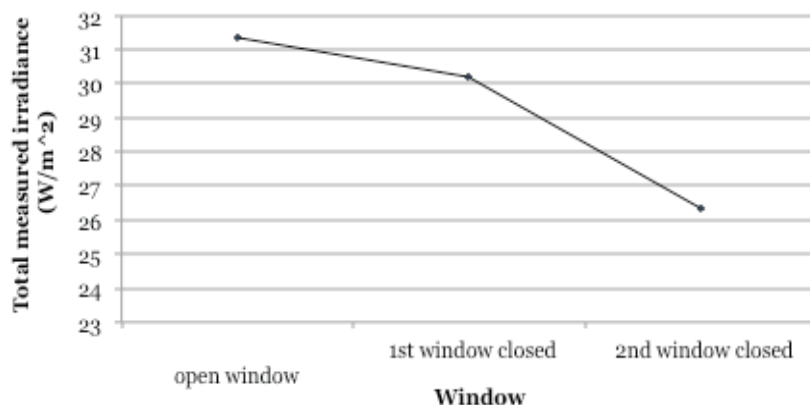
FIGURE C1.4: TOTAL MEASURED IRRADIANCE ( \text{W/m}^2 ) AT DISTANCE 2 CM FROM THE WINDOW AT A NORTH ORIENTED OFFICE, AT DELFT, THE NETHERLANDS ON JUNE 10TH, 2015. THE WINDOW IS DOUBLE-GLAZING. WE MEASURE IRRADIANCE WITH WINDOW OPEN, 1ST WINDOW CLOSED AND BOTH WINDOWS CLOSED. WE AIM TO INVESTIGATE THE TRANSMITTANCE OF THE WINDOW. THE THREE MEASUREMENTS TOOK PLACE WITH TIME DELAY OF 1 MIN BETWEEN EACH OTHER.
