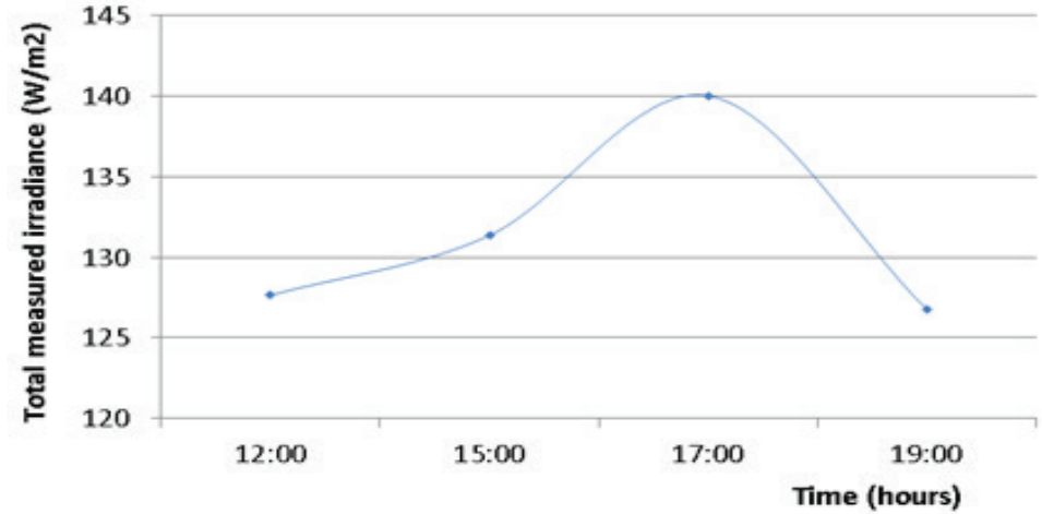
FIGURE C1.8: TOTAL MEASURED IRRADIANCE ( \text{W/m}^2 ) ON 28.03.2012 AT A NORTH ORIENTED OFFICE, SENSOR'S POSITION N1, DELFT.
