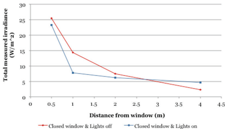
FIGURE 4.19: TOTAL MEASURED IRRADIANCE ( \text{W}/\text{m}^2 ) AT A SOUTH-FACING OFFICE ON JUNE 10TH, 2015, AT DELFT, THE NETHERLANDS. IN BOTH CASES THE WINDOW WAS CLOSED DURING THE MEASUREMENTS, WHILE THE LIGHTS WERE ON FOR THE BLUE LINE AND OFF FOR THE RED ONE.
