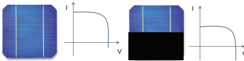
FIGURE 2.6: EFFECT ON THE OUTPUT CURRENT, WHEN PART OF THE PV MODULE IS SHADED (ADAPTED FROM HONSBURG AND BOWDEN, 2015).
