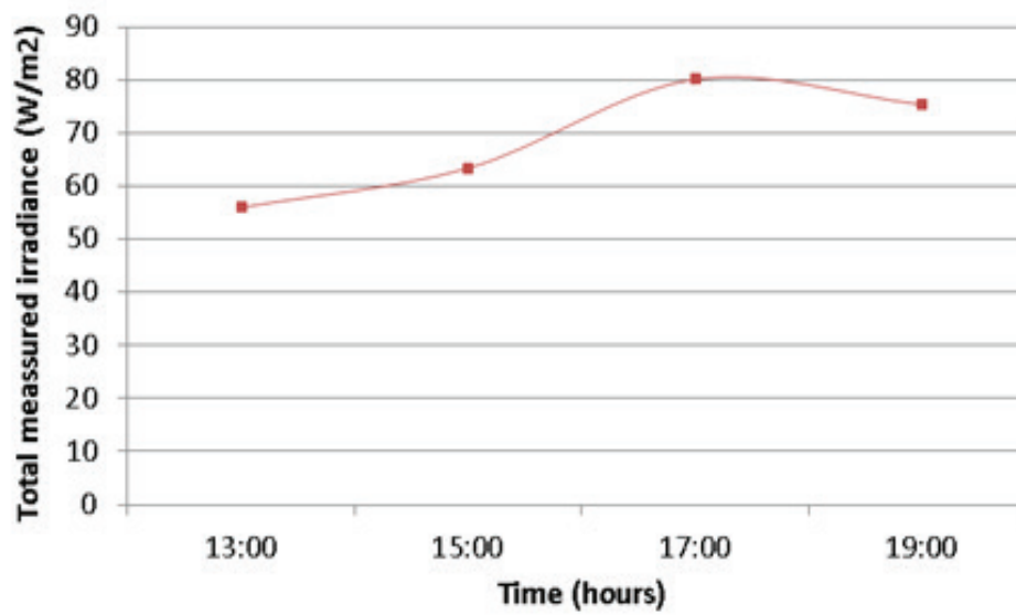
FIGURE C1.10: TOTAL MEASURED IRRADIANCE ( \text{W/m}^2 ) ON 04.04.2012 AT A NORTH ORIENTED OFFICE, SENSOR'S POSITION N3, TU DELFT.
