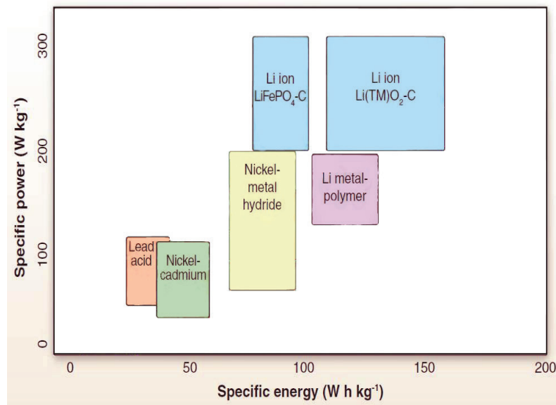
FIGURE 2.8: GRAVIMETRIC POWER AND ENERGY DENSITIES FOR DIFFERENT RECHARGEABLE BATTERIES (ADAPTED FROM DUNN, ET AL., 2011).
