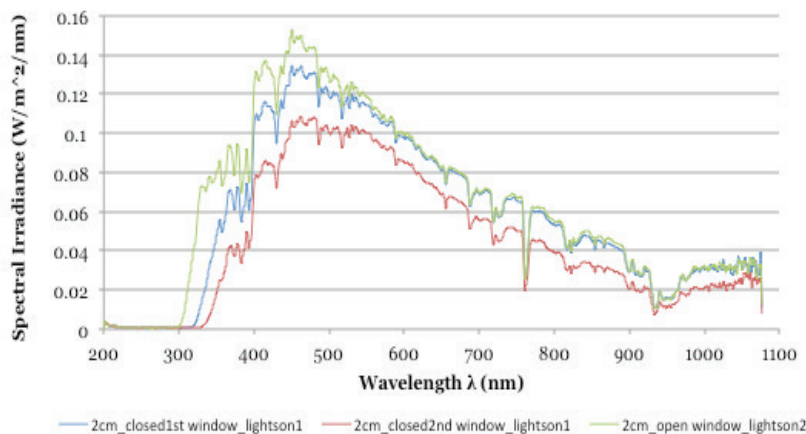
FIGURE C1.6: SPECTRAL IRRADIANCE ( \text{W/m}^2/\text{nm} ) MEASURED AT DISTANCE 2 CM FROM THE WINDOW AT A SOUTH ORIENTED OFFICE AT DELFT, THE NETHERLANDS, ON JUNE 10TH, 2015.
