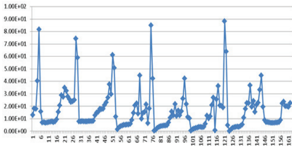
FIGURE C2.3: TOTAL RADIANT POWER IN ( \text{W}/\text{m}^2 ) FOR ONE WEEK OF CONTINUOUS MEASUREMENTS PER HOUR. THE X-AXIS REPRESENTS THE NUMBER OF MEASUREMENTS; 1 IS THE FIRST MEASUREMENT, WHICH CONDUCTED ON APRIL 30TH, 2015 AT 15:00 AND THE 161 IS THE LAST MEASUREMENT ON MAY 7TH, 2015 AT 7:00. THE PACE OF THE SPECTRORADIOMETER IS 60 MINUTES BETWEEN TWO MEASUREMENTS. THE Y-AXIS IS THE MEASURED TOTAL RADIANT POWER IN \text{W}/\text{m}^2 .
