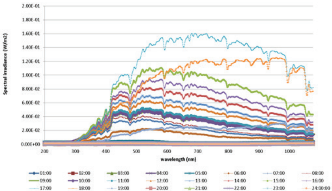
FIGURE C2.1: SPECTRAL IRRADIANCE MEASUREMENTS ( \text{W/m}^2/\text{nm} ) ON 21.01.2014, AT A NORTH ORIENTED OFFICE AT TU DELFT.
