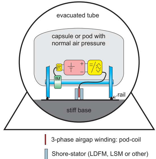
Fig. 2. Sketch of pod on wheels from the rear with linear motor and a speed-keeper motor. The different shore-stator types are sketched in figures 3 and 4.
