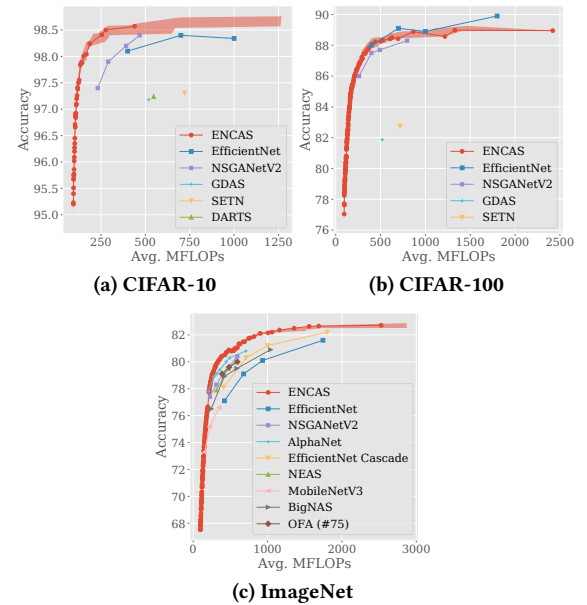
Figure 6: Comparing ENCAS with SOTA NAS algorithms.
