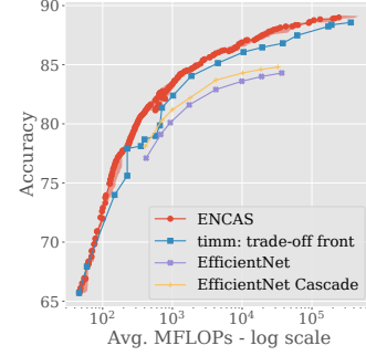
Figure 8: ENCAS discovers a dominating trade-off front on ImageNet by searching for cascades of 518 timm models (from which only the models on the trade-off front are shown).
