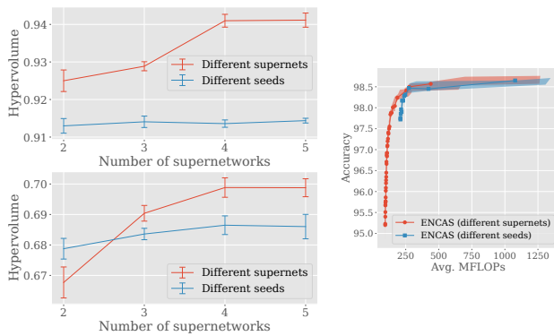
Figure 10: Comparison between hypervolume when using different supernetworks, or the best supernetwork trained with different seeds on (top left) CIFAR-10, (bottom left) CIFAR-100. (right) shows comparison between trade-off fronts of 5 supernetworks, or 5 seeds of the best supernetwork on CIFAR-10.
