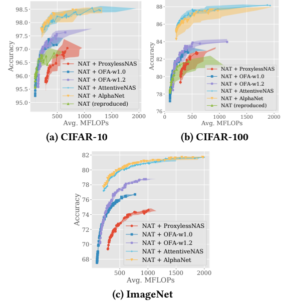
Figure 4: Results of running NAT [27] with different supernetworks on CIFAR-10, CIFAR-100, ImageNet.
