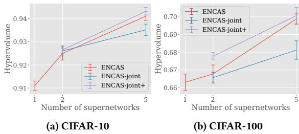
Figure 9: Impact of increasing the number of supernetworks in ENCAS, ENCAS-joint, ENCAS-joint+.
