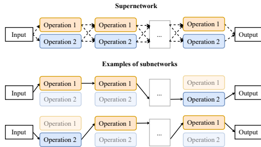
Figure 1: A schematic of a generic supernetwork.
