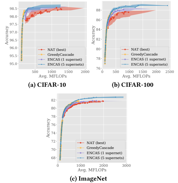
Figure 5: Comparing ENCAS to the baselines.
