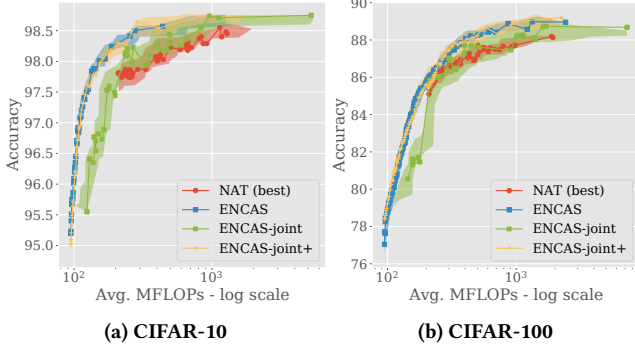
Figure 7: Investigating benefits of joint training and search.
