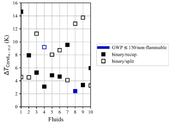
Fig. 7. \Delta T_{cond,H-VLE} for selected fluids. Fluid number identifier in Table 5.
