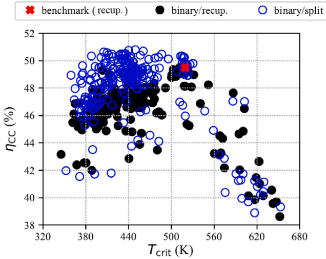
Fig. 5. Comparison of \eta_{cc} over T_{crit} .
