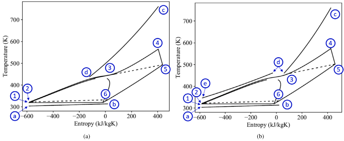
Fig. 2. T - s -diagram representation of the processed forming the recuperated-cycle (a) and split-cycle (b) configurations in case R245fa is the working fluid; The thermodynamic state numbering is consistent with that of Fig. 1.
