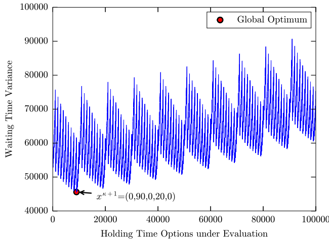
Figure 3. Evaluating |q|^{|x_m|} = 10^5 = 100,000 bus holding options with Brute Force. The globally optimal solution is (0, 90, 0, 20, 0) sec with a performance of 45,571.03 \text{ s}^2 .
