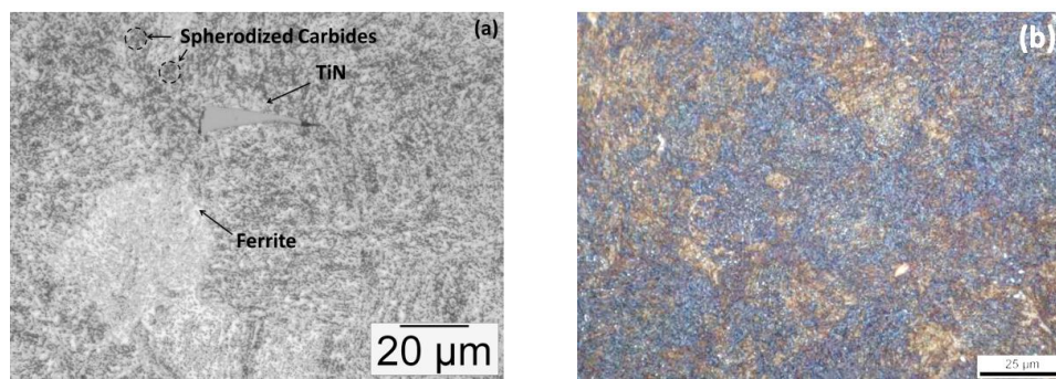
Figure 4. (a) Initial microstructure of the CrMo steel in the soft annealed condition (b) Microstructure of the CrMo steel after UFHT. Blue and brown regions indicate the appearance of bainite and martensite, respectively, while white areas indicate the existence of carbides (or possibly retained austenite).
