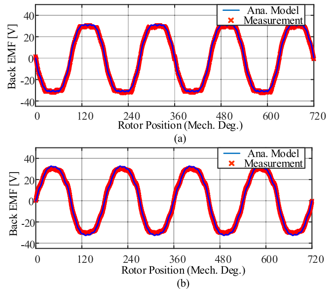
Fig. 20. EMFs results. (a) Normal. (b) Partial demagnetization.
