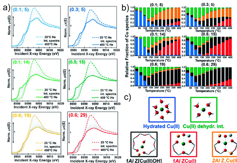
Figure 15. (a) In situ XANES of Cu-CHA catalysts with different compositions (different samples are denoted with (Cu/Al; Si/Al) labels) during dehydration under He flow from 25 to 400 °C, heating rate 5 °C min -1 . (b) Temperature-dependent abundance of pure Cu species in each of the catalysts as derived from multivariate curve reconstruction based on alternating least-squares (MCR-ALS) analysis of global temperature-dependent XANES data set collected for six Cu-CHA samples. (c) Proposed assignment of the five pure components to specific Cu species/sites formed in the Cu-CHA catalyst as a function of composition and activation temperature, using the same color code as in part (b). Blue (PC1): mobile Cu(II)-aquo-complexes [Cu(II)(H 2 O) n ] 2+ /[Cu(II)(H 2 O) n-1 (OH)] + with n = 6; green (PC5): Cu(II) dehydration intermediate, possibly represented by mobile [Cu(II)(H 2 O) n ] 2+ /[Cu(II)(H 2 O) n-1 (OH)] + complexes with n = 4; black (PC3): 1Al Z[Cu(II)OH] sites in their oxidized form; red (PC2): 1Al ZCu(I) sites in their reduced form, resulting from self-reduction of 1Al Z[Cu(II)OH] species; orange (PC4): 2Al Z 2 Cu(II) sites. Atom color code: Cu: green; H: white; O: red; Si: gray; Al: yellow. Adapted with permission from ref 214. Copyright 2017 The Royal Society of Chemistry.
