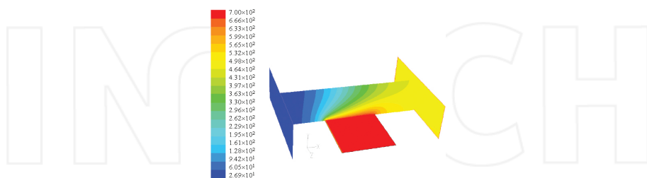
Figure 1. Temperature distribution profile simulated by commercial FLUENT ® software for an ASM Epsilon One CVD reactor when the total pressure is ATM. The hydrogen gas is considered to be the main gas flowing over the susceptor, in order to simplify the simulation. The susceptor is heated up by an assembly of lamps to the deposition temperature (here 700°C) [19].
