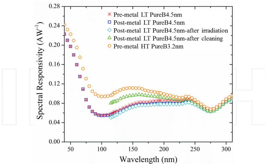
Figure 15. Measured VUV spectral responsivity as a function of wavelength for HT and LT PureB photodiodes (area: 9.6×9.6 mm 2 ) before and after high-level irradiation and after a final cleaning procedure [22].
