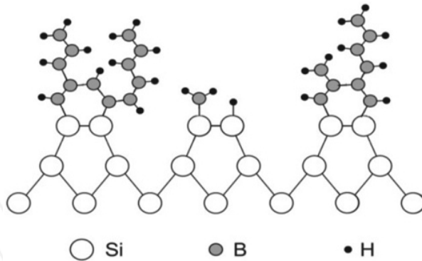
Figure 6. Schematic of the deposition of the first few monolayers of boron layers for (a) HT, 700°C, and (b) LT, 400°C, deposition when an Si surface is exposed to B_2H_6 [22].
