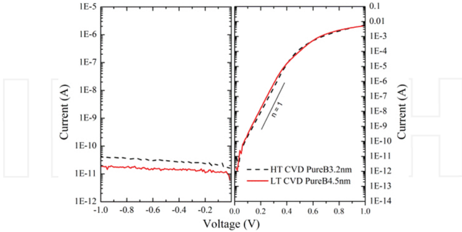
Figure 14. Measured I-V characteristics of both pre-metal HT and post-metal LT PureB photodiodes with an active area of 9.6×9.6 mm 2 . Schematics of the fabricated photodiodes are shown in Figure 13 . The boron layer thickness was measured by ellipsometry to be 3.2 and 4.5 nm for the HT and LT photodiodes, respectively [25].
