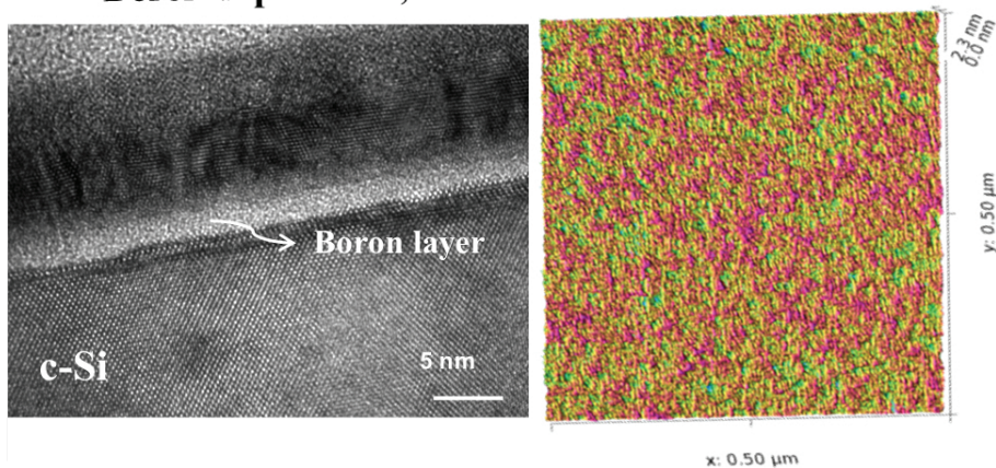
Figure 5. HRTEM image (left) and atomic-force microscopy (AFM) measurement (right) of a 6-min HT-deposited boron layer surface. The AFM image was taken in a 500×500 nm 2 scanning area. This HT layer is smooth and uniform at a thickness of about 2 nm with a root-mean-square (rms) roughness value of 0.204 nm [21].
