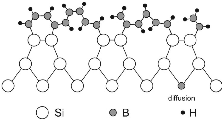
Figure 4. Schematic of the deposition of the first few monolayers of boron layers for HT, 700^{\circ}\text{C} , deposition when a Si surface is exposed to \text{B}_2\text{H}_6 [22].
