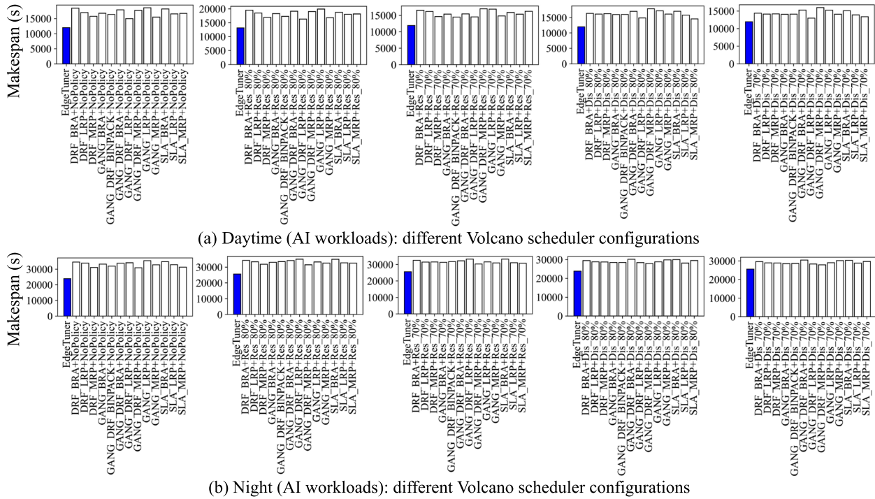
Fig. 11 Comparison of Makespan under AI workloads driven by Alibaba trace 2020
