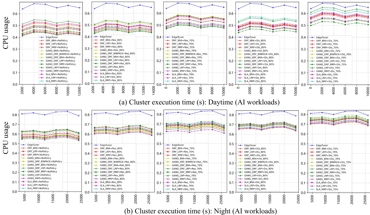
Fig. 12 Average CPU usage of the cluster during a certain execution period under AI workloads
