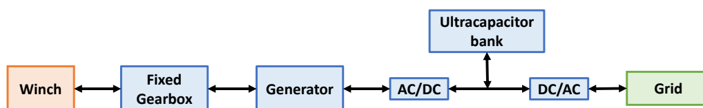
Figure 4: Architecture of a fully electric power smoothing solution
