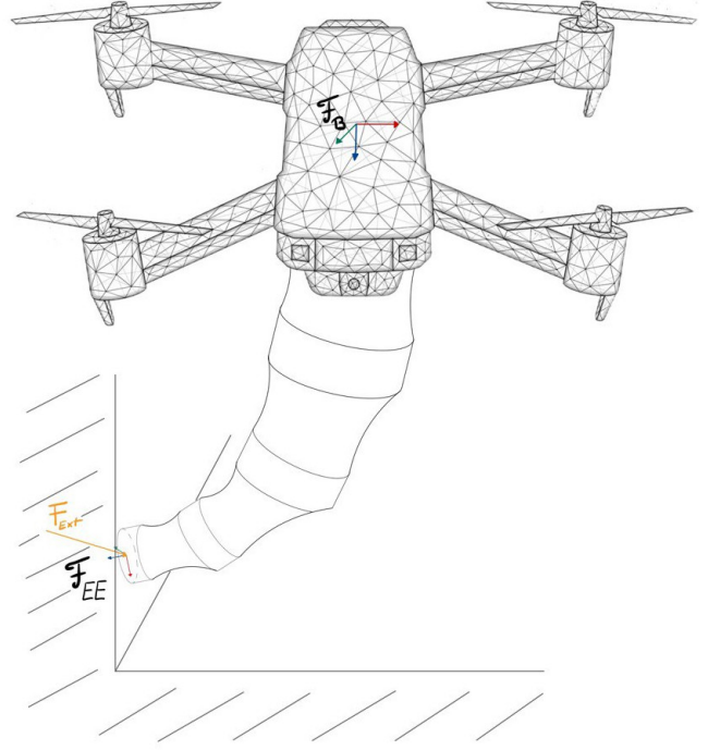
Fig. 1: A UAV equipped with a compliant finger in contact with its surroundings. From measuring the manipulator state the contact force can be estimated and used for force control to maintain contact with the environment.
