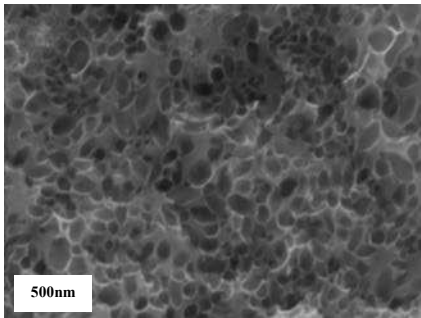
Figure 1. CNNs precursor
