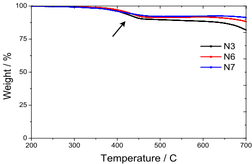
Figure 5. Thermogravimetric Analysis
