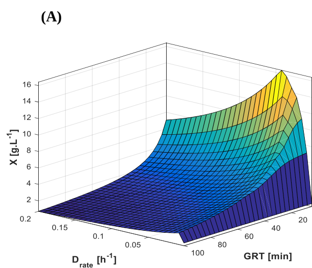
Figure A2-6. Steady-state cell mass concentration as function of gas residence time (GRT) and liquid dilution rate ( D_{rate} ): (A) with 90% cell recycle; (B) without cell recycle. Fixed conditions: y_{CO} = 0.65 , y_{H_2} = 0.2 , y_{CO_2} = 0.15 and N = 500 rpm.
