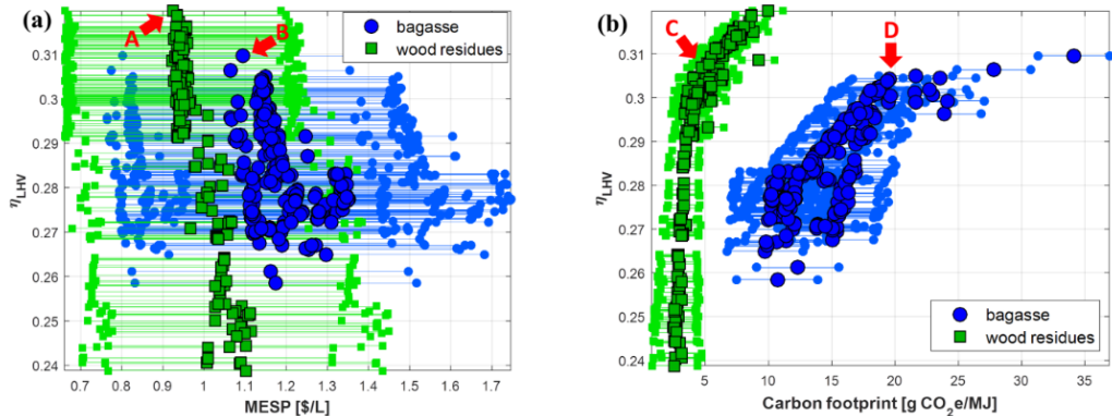
Figure 5.11. Projections of 3-objective Pareto fronts in pairs, including intervals of \pm 30\% uncertainty in economic and environmental assumptions: (a) MESP; (b) Carbon footprint.
