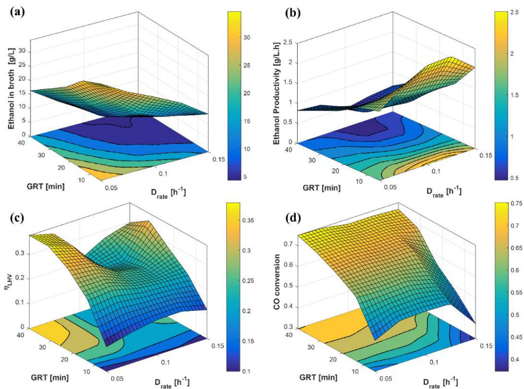
Figure 5.7. Bubble column reactor, sensitivity of D_{rate} and GRT on model outcomes: (a) ethanol concentration [ g \cdot L^{-1} ] in the liquid phase; (b) ethanol productivity [ g \cdot L^{-1} \cdot h^{-1} ]; (c) energy efficiency \eta_{LHV} ; (d) CO conversion.
