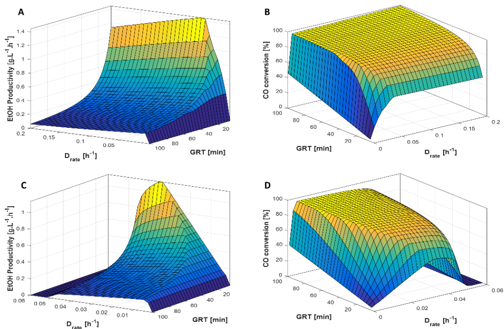
Figure 3.6. Steady-state ethanol productivity and CO conversion as function of gas residence time (GRT) and liquid dilution rate ( D_{rate} ): (A, B) with 90% cell recycle; (C, D) without cell recycle. Fixed conditions: y_{CO} = 0.65 , y_{H_2} = 0.2 , y_{CO_2} = 0.15 , N = 500 rpm. Note: the axes are rotated in (A) and (C).
