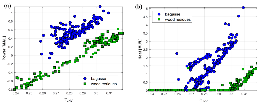
Figure 5.14. Pareto-optimal values of global energy balance (consumed minus produced in the plant): (a) power; and (b) heat (steam).
