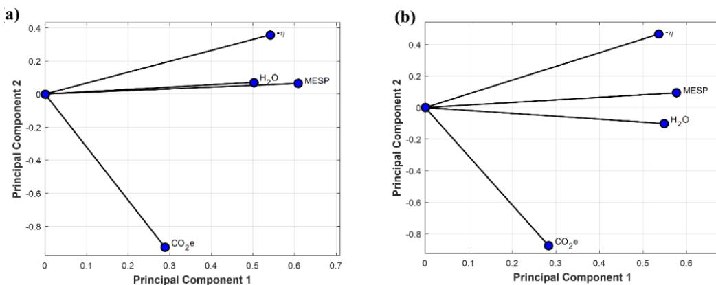
Figure 5.9. PCA of model responses showing the principal component coefficients (loadings) of the first two principal components: (a) sugarcane bagasse; (b) wood residues.
