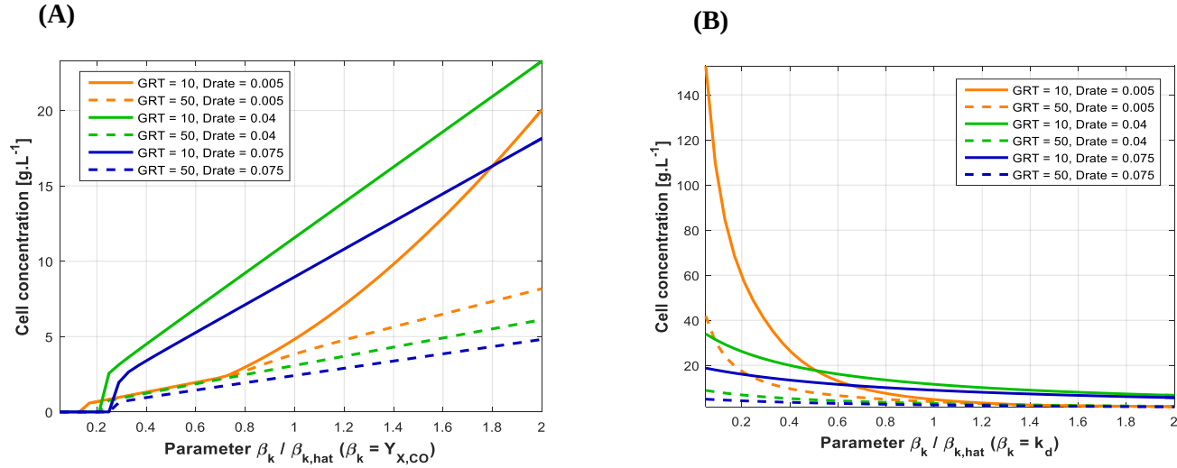
Figure A2-7. Sensitivity of steady-state cell mass concentration to kinetic parameters under different conditions of gas residence time ( GRT ) and liquid dilution rate ( D rate ): (A) cell yield on CO ( Y_{X/CO} ); (B) cell death rate constant ( k_d ). Fixed conditions: y_{CO} = 0.65 , y_{H_2} = 0.2 , y_{CO_2} = 0.15 and N = 500 rpm.
