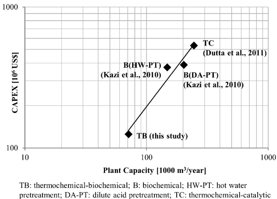
Figure 2.4. Comparison of CAPEX estimate with other studies. CAPEX results from other works were adjusted to 2015 prices.
