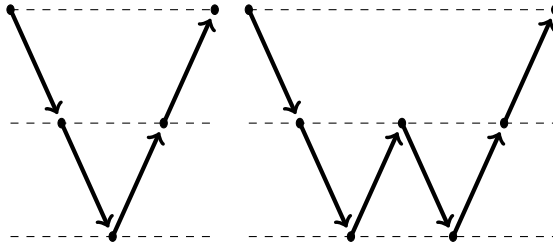
Figure 3.1: Description of a V-cycle (left) and W-cycle (right).
