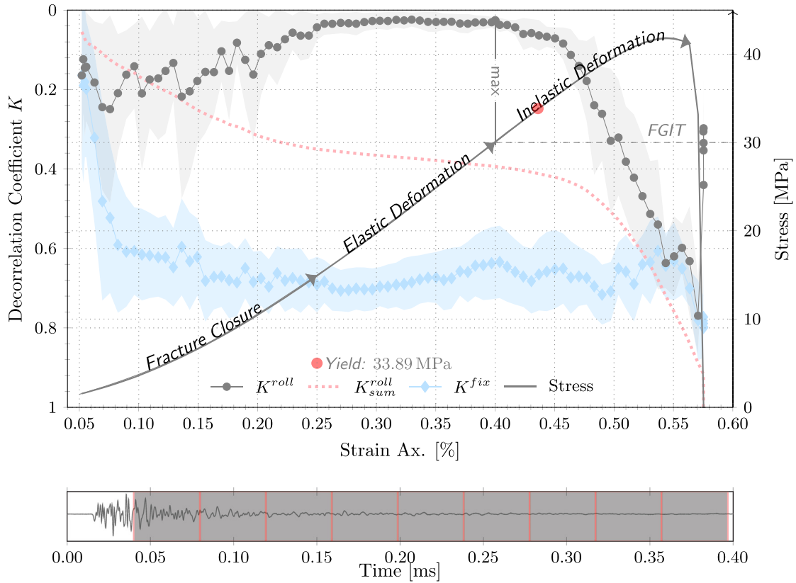
FIG. 2. (Color online) CWD monitoring (receiver 2) of BNT1. The mean fixed reference decorelation coefficient K^{fix} is compared with the rolling reference equivalent K^{roll} and its cumulative sum K^{roll}_{sum} , calculated from the 9 independent correlation windows. The K^{roll} trend is generated with a rolling lag equal to the repeat measurement period of 15 s (i.e., N = 1 ), from which the FGIT is identified at 30 MPa. The shaded area represents the standard deviation about the mean decorelation as calculated from the 0.04 ms correlation windows shown over a single waveform.
