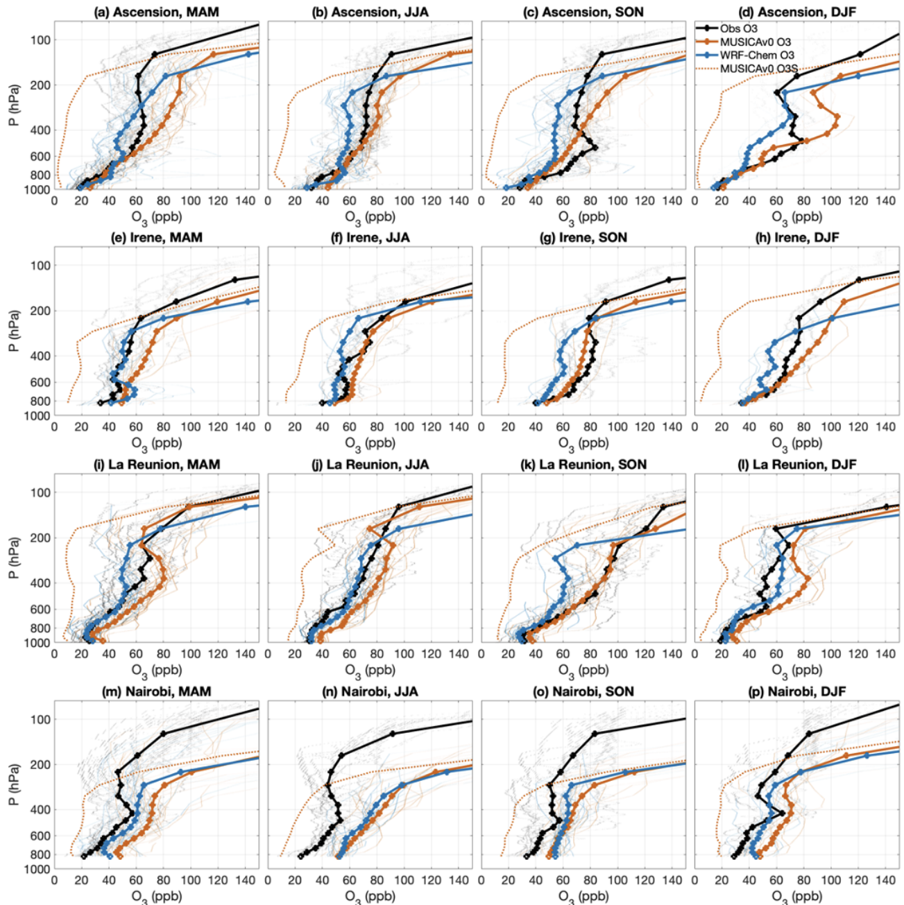
Figure 10. Vertical profiles of \text{O}_3 (ppb) from ozonesondes (black) and corresponding model output from MUSICAv0 (red) and WRF-Chem (blue) for each season of 2017. The thick lines denote the seasonal mean profiles and the thin lines denote the individual profiles. The dashed red lines represent \text{O}_3\text{S} (stratospheric ozone tracer) from the MUSICAv0 simulation. Ozonesonde data at Ascension in (a) MAM (March, April, and May), (b) JJA (June, July, and August), (c) SON (September, October, and November), and (d) DJF (December, January, and February) are shown. Panels (e)–(h), (i)–(l), and (m)–(p) are the same as (a)–(d), except for Irene, La Réunion, and Nairobi, respectively. Locations of the sites are shown in Fig. 1b.
