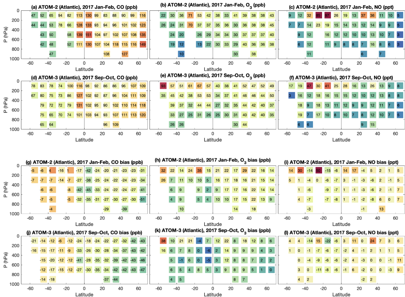
Figure 12. Observations of (a) CO (ppb), (b) O 3 (ppb), and (c) NO (ppt) over the Atlantic Ocean during ATom-2 and ATom-3 (d–f). (g–l) Corresponding model biases against ATOM observations. The ATom airborne measurements and corresponding MUSICA v0 model results are binned to 10° latitude and 200 hPa pressure bins. The values of mean biases for each latitude and pressure bin are labeled in the figure.
