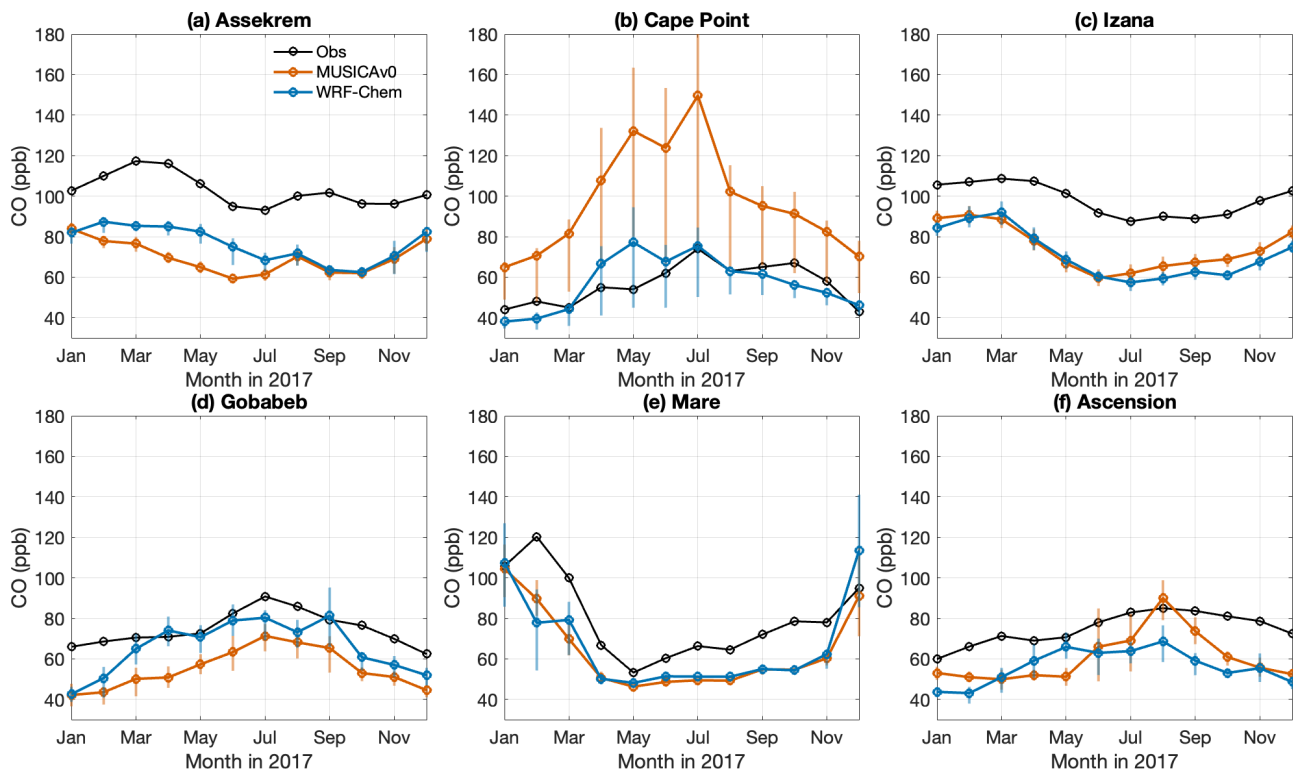
Figure 6. Monthly mean CO (ppb) from in situ observations (black), MUSICA v0 (red), and WRF-Chem (blue) during 2017 at (a) Assekrem, (b) Cape Point, (c) Izaña, (d) Gobabebe, (e) Mare, and (f) Ascension (see Fig. 1b for locations). Monthly means are calculated from 3-hourly data. The range for each data point shows the variation in the 3-hourly data on that day (25 % quantile to 75 % quantile). Observational data are from the World Data Centre for Greenhouse Gases (WDCGG).
