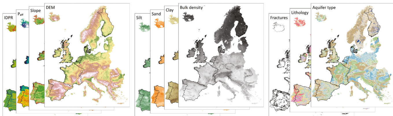
Fig. 2. Illustration of the range of covariates used for the machine learning predictions of recharge coefficients. The seven countries providing training data on recharge coefficients are outlined with black boundaries.
